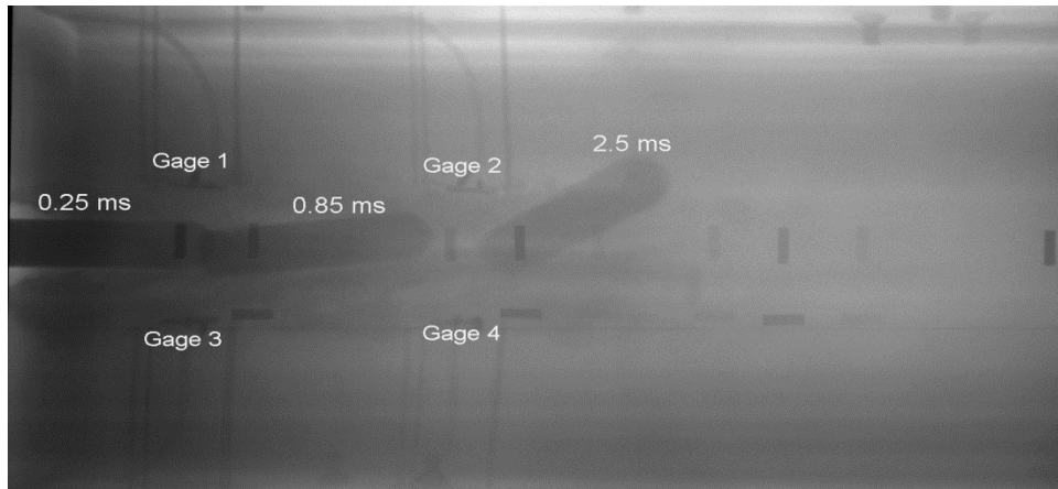
Figure 8: Projectile deflects away by sensors below the shot line.
