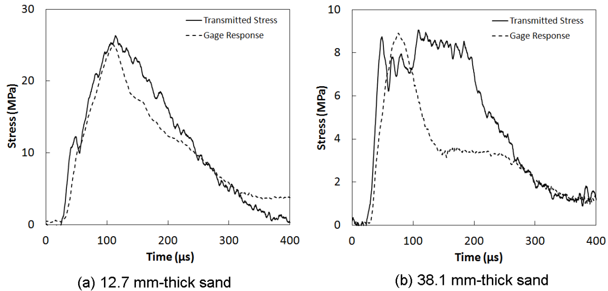
Figure 22: Comparison of gauge output and bar signals.
