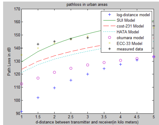
Fig.2 Comparison of path loss models with measurements from an urban environment
