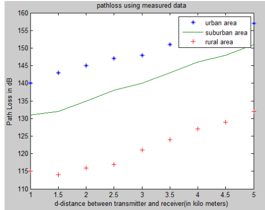
Fig.1 Measured path loss in different environment
