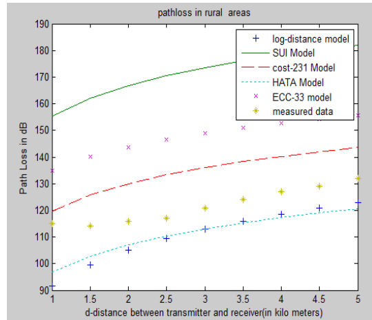
Fig.4 Comparison of path loss models with measurements from a rural environment
