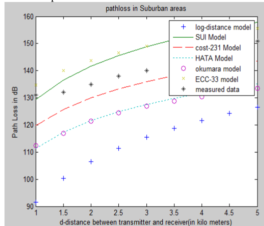
Fig.3 Comparison of path loss models with measurements from a suburban environment
