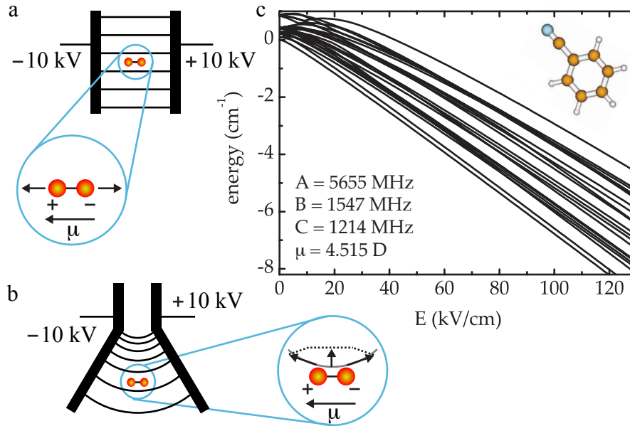
Figure 10: a) Homogeneous electric fields can be used to orient polar molecules. The field does not provide an overall (translational) force on the molecule, but it provides a torque to orient the molecular dipole moment along the electric field lines. b) Inhomogeneous electric fields exert a force on polar molecules: the centers of positive and negative charge do not coincide and, therefore, the forces on these charge-centers do not cancel exactly. Instead, a small remaining force, depicted by the vectorial sum in the inset, remains and can be used to manipulate the translation of the molecule. c) Potential energy as a function of the electric field strength for the lowest rotational quantum states of benzonitrile. These energies can be calculated from the spectroscopically determined rotational constants A , B , C and the dipole moment \mu . 148
