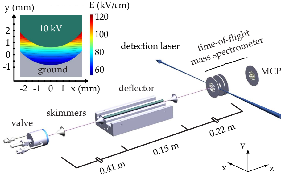
Figure 1: Sketch of the experimental setup for electric beam deflection. In the inset, a cut through the deflector is shown, and a contour plot of the electric field strength is given.
