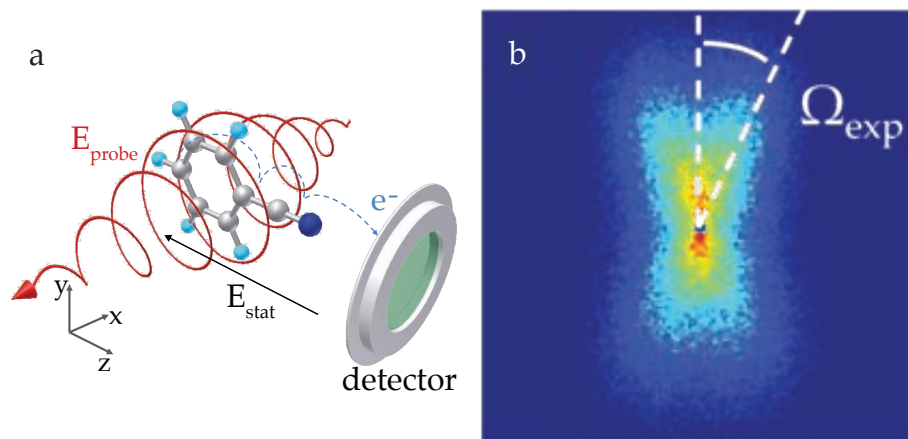
Figure 7: Molecular-frame photoelectron-angular-distribution imaging schematics (a) and the corresponding molecular-frame photoelectron angular distribution of 3D oriented benzonitrile molecules; 121 see text for details.
