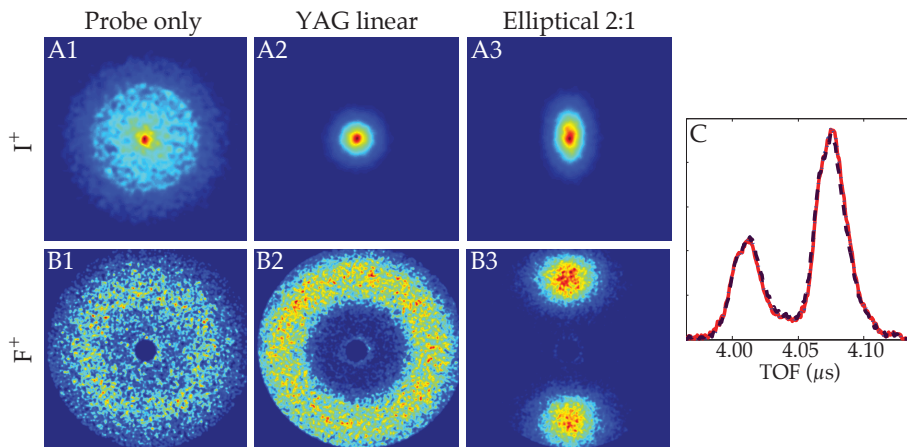
Figure 6: Velocity-map images (A1-B3) and time-of-flight distributions (C) of difluoroiodobenzene. Images A1–A3 show the velocity distribution of iodine ions, B1-B3 of fluorine ions for isotropic (A1, B1), 1D oriented (A2, B2) and 3D oriented (A3, B3) difluoroiodobenzene molecules. The scales of these images can be calibrated by calculation of the Coulomb repulsion force in the fragmenting molecule, but these scales are not relevant for the discussion of alignment and orientation. The time-of-flight distribution of iodine ions represents the forward-backward asymmetry of the 3D oriented sample (reproduced from reference 120).
