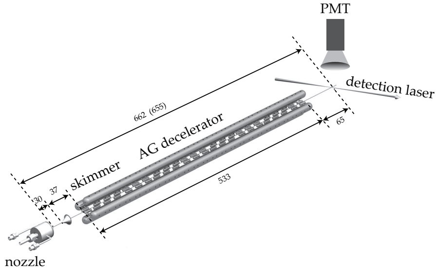
Figure 3: Sketch of the experimental setup for alternating gradient deceleration consisting of a pulsed valve, a skimmer, the \sim 0.5 m long decelerator module, and a quantum-state resolving laser-induced-fluorescence detection setup using a photomultiplier tube (PMT).
