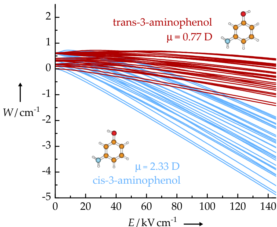
Figure 4: Molecular structures, dipole moments, and energies of the lowest rotational states of cis- and trans-3-aminophenol as a function of the electric field strength (reproduced from reference 42).
