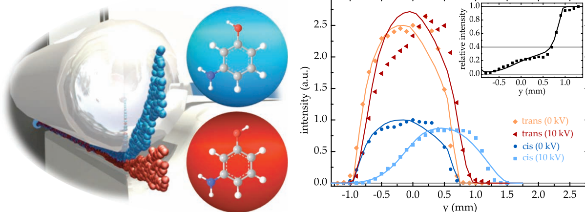
Figure 5: Conformer separation by deflection. The sketch on the left illustrates the spatial separation of the conformers of 3-aminophenol in a molecular beam entering the device through a skimmer from the back. The figure on the right shows an actual measurement of the vertical beam profiles. These profiles can be independently obtained, for example, through resonance-enhanced multi-photon ionization, which spectrally discriminates the two species. The inset shows the relative abundance of the trans conformer as a function of vertical position in the deflected molecular beam (reproduced from reference 42).
