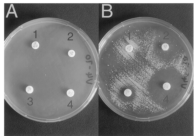
Figure 2. Satellitism of Staphylococcus aureus (case no. 70) around \beta -lactam antibiotic disks on Mueller-Hinton agar plates with 4 \mu\text{g}/\text{mL} vancomycin. A , Agar plate without addition of NaCl; B , agar plate with the addition of 4% NaCl. 1 = aztreonam; 2 = ceftibuten; 3 = oxacillin; 4 = cefoxitin.
