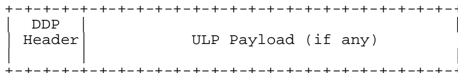
Figure 6 DDP Segment Format
