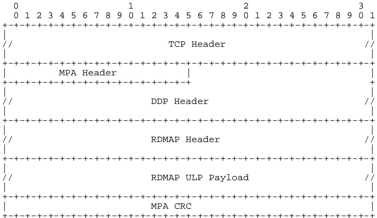
Figure 2 MPA, DDP, and RDMAP Header Alignment
