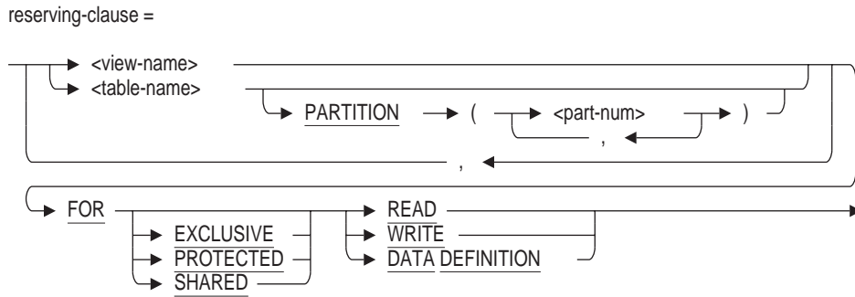
Figure 10–1 RESERVING Clause
