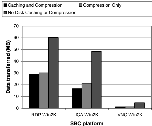
Figure 3 Effect of caching and compression
