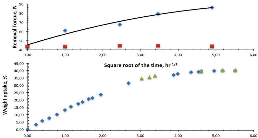
Figure 5. Comparison between the kinetics of after implantation removal torque increases and physiological fluid uptakes in modified implants undergoing swelling.
