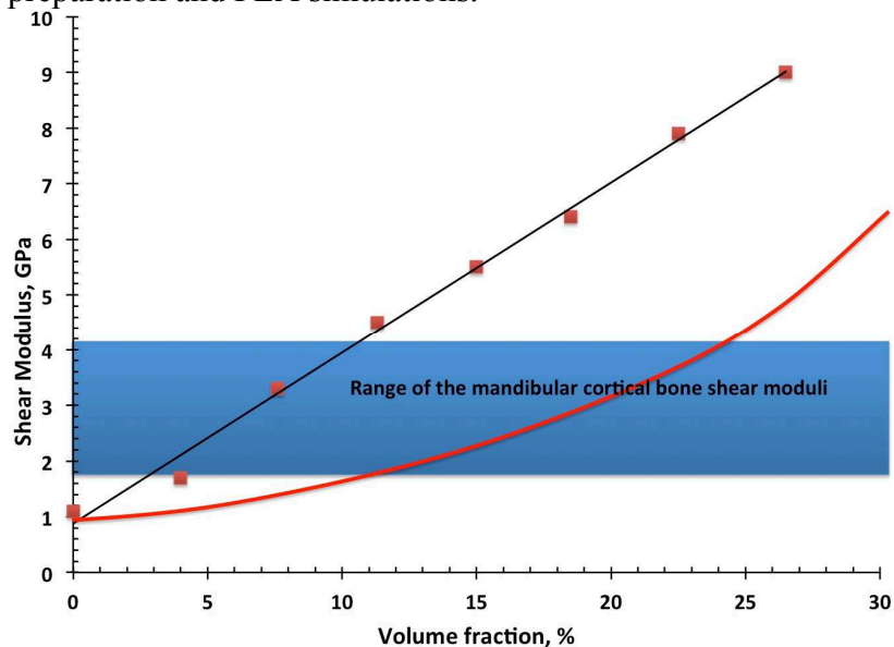
Figure 1. Shear moduli of the hybrid nanocomposites at different nanosilica filler loading. The theoretical Halpin-Tsai curve is reported for comparison in the figure.
