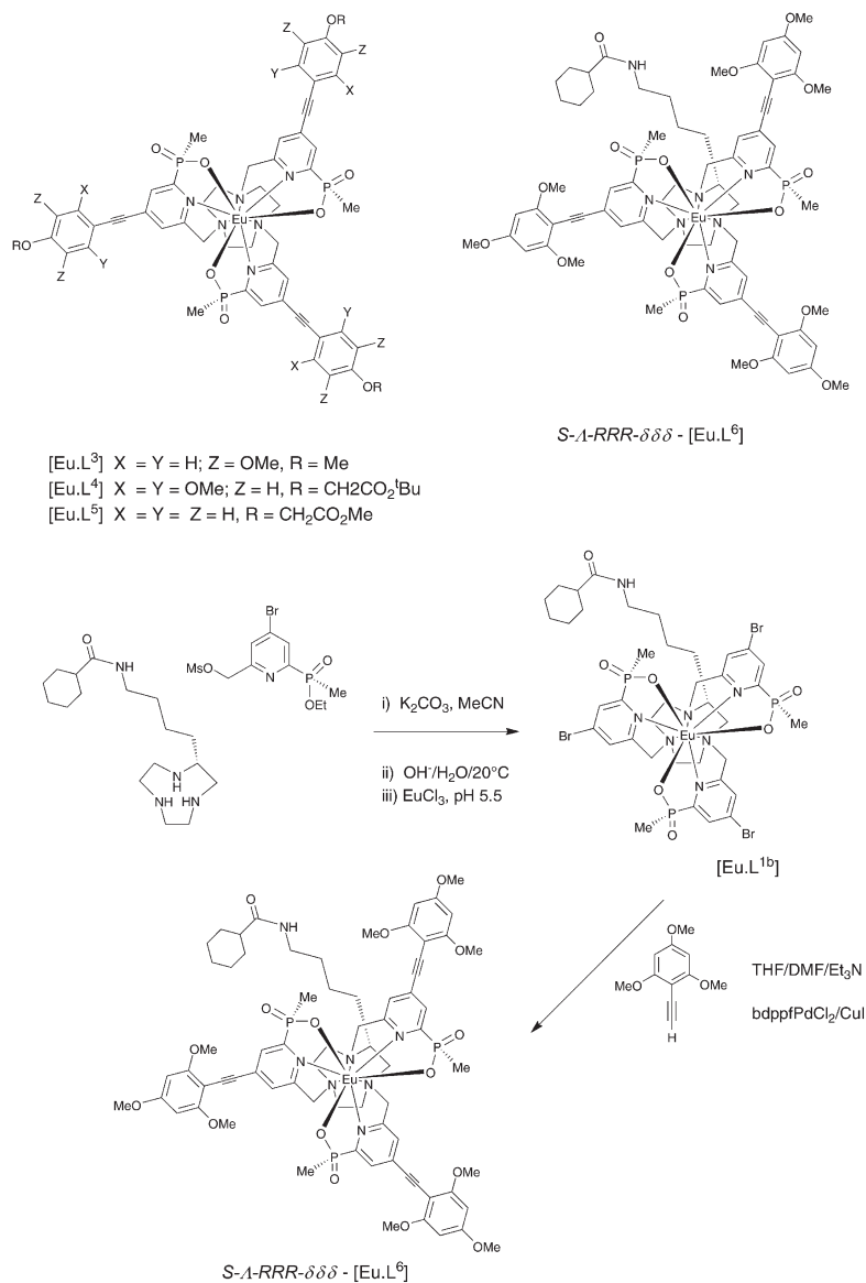
Scheme 2 Synthesis of the enantiopure complex [Eu.L 6 ].
