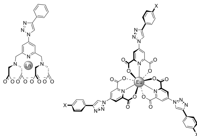
Fig. 2 Selected reported pyridyl-triazole-aryl lanthanide complexes. 21,22
