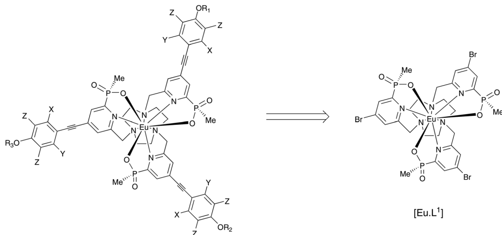
Fig. 1 Retrosynthetic analysis of tris-pyridyl-alkynyl-aryl phosphinate complexes.
