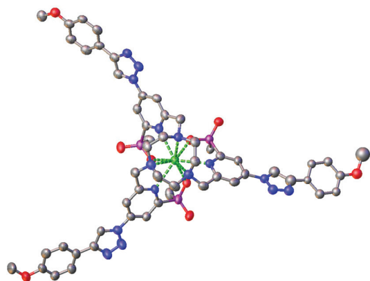
Fig. 3 The molecular structure of [\text{Eu}\cdot\text{L}^2] (ellipsoids are drawn at the 50% probability level; one of the disordered components and the H atoms are omitted for clarity: CCDC 982687).
