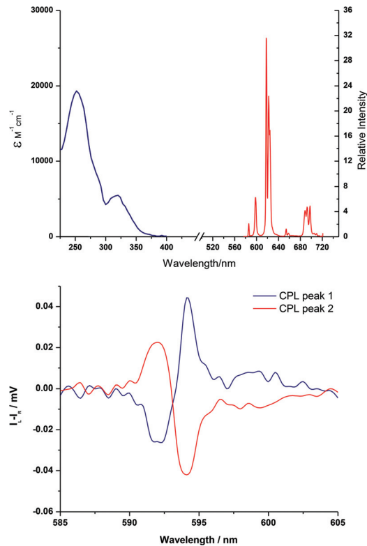
Fig. 5 Upper: Absorption and emission spectra of [Eu-L 2 ], (MeOH, 295 K); lower: CPL spectrum of the \Delta J = 1 region showing near mirror image spectra of the \Delta (blue: eluting first) and \Lambda (red) enantiomers (n.b. photobleaching occurred during data acquisition, leading to a loss of sensitivity: 10 scans were recorded (1 min each) and summed; [complex] = 110 \mu mol).
