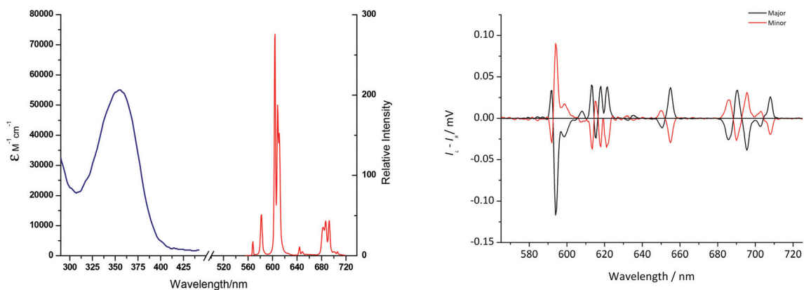
Fig. 6 Left: absorption and total emission spectrum of [Eu.L 6 ]; right: circularly polarised emission spectra of (major/black) S -RRR- \Lambda -[Eu.L 6 ], (MeOH, 295 K, 3 \mu M, 20 min; g_{em} = +0.30 (708 nm); +0.17 (655 nm); -0.11 (598 nm)), and the enantiomeric \Delta -complex (red/minor) with an R stereogenic centre at C.
