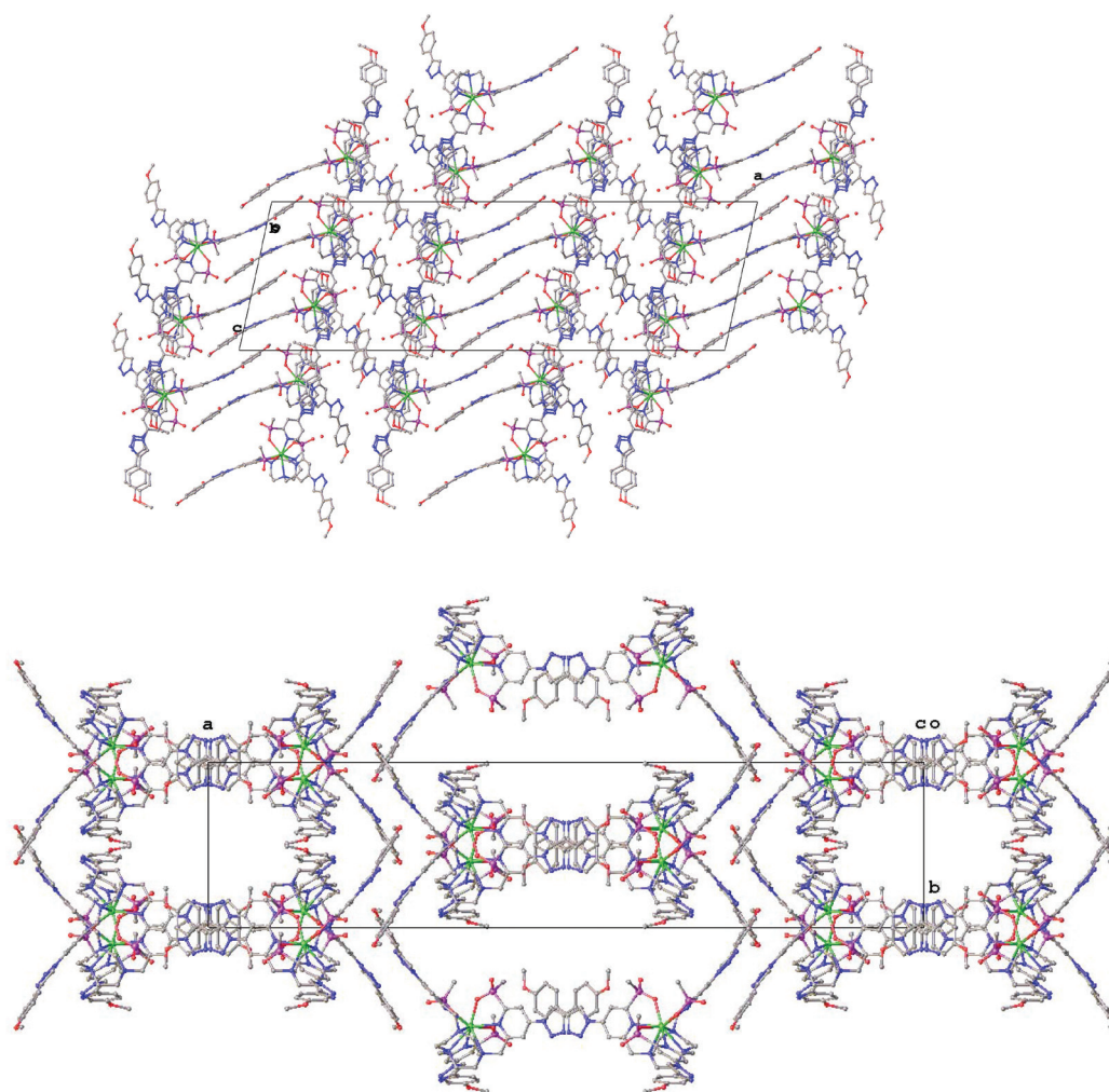
Fig. 4 Views of the packing of [\text{Eu}\cdot\text{L}^2] in the crystal lattice (100 K), showing the channels in the lattice arising from \pi -stacking of the aryl-substituted chromophores.
