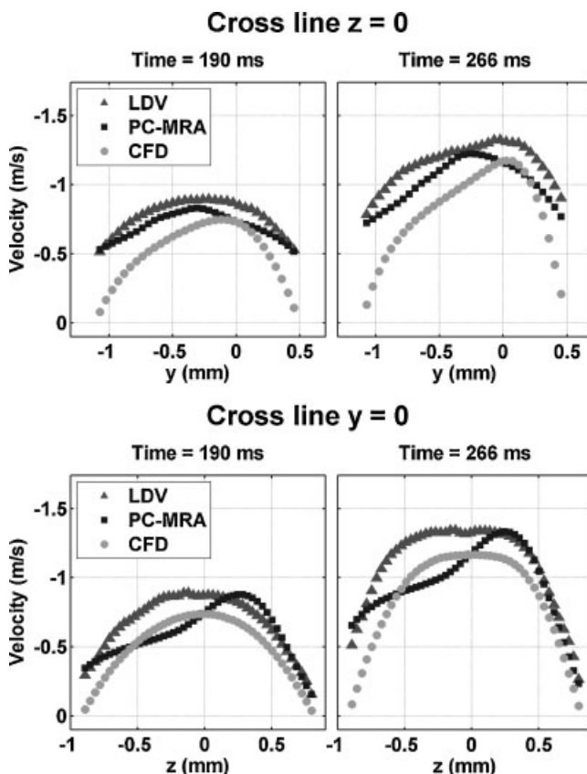
Figure 9. The profile lines of the through-plane velocities at the anterior cerebral artery show similar patterns, except in the peak flow region.
