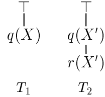
Figure 4: The tableaux from Example 3.4.
