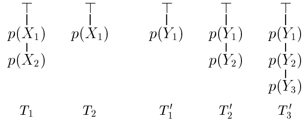
Figure 3: The tableaux from Example 3.3.
