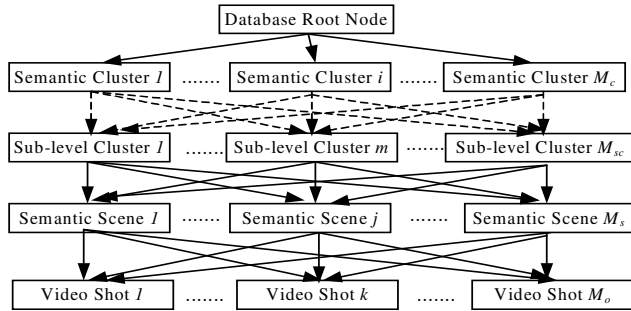
Figure 1. The proposed hierarchical video database model
