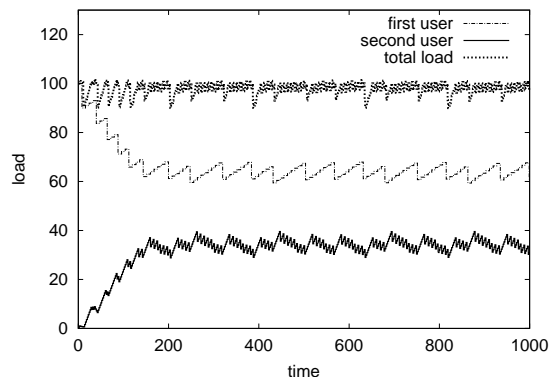
(b) convergence from the unfair efficient state
