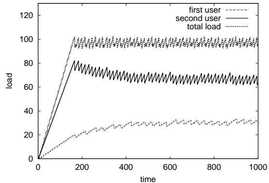
(a) convergence from the fair inefficient state
