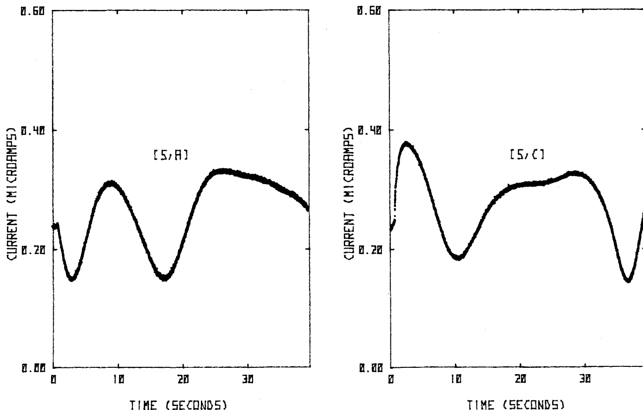
Fig. 14. Limiting current to segments before and after the disengagement of a bubble. (a, left; b, right)
