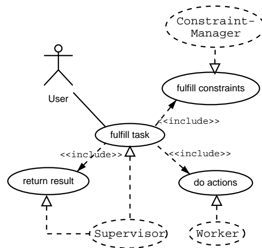
Figure 3: Use-Case diagram of the problem
