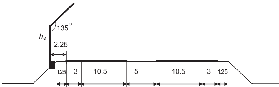
Figure 4. Location of noise barriers. Notes. h_e —height of acoustic screen.
