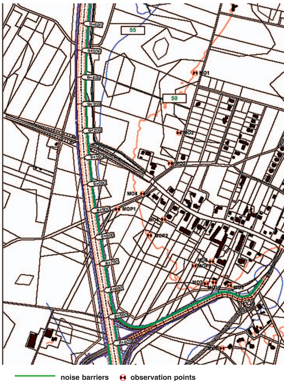
Figure 3. Sample noise calculations for Wrocław's motorway ring-road—with designed barriers.
