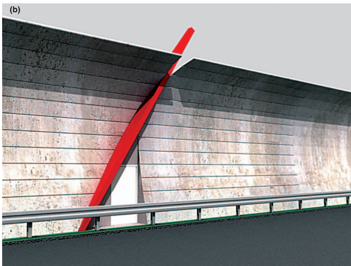
Figure 5. WMRR noise barriers—architectural elements: (a) a change in barrier type or height, (b) an emergency exit. Notes. WMRR—Wrocław’s motorway ring-road. Design: Paweł Ogielski, visualisation: Jakub Chojnacki.
