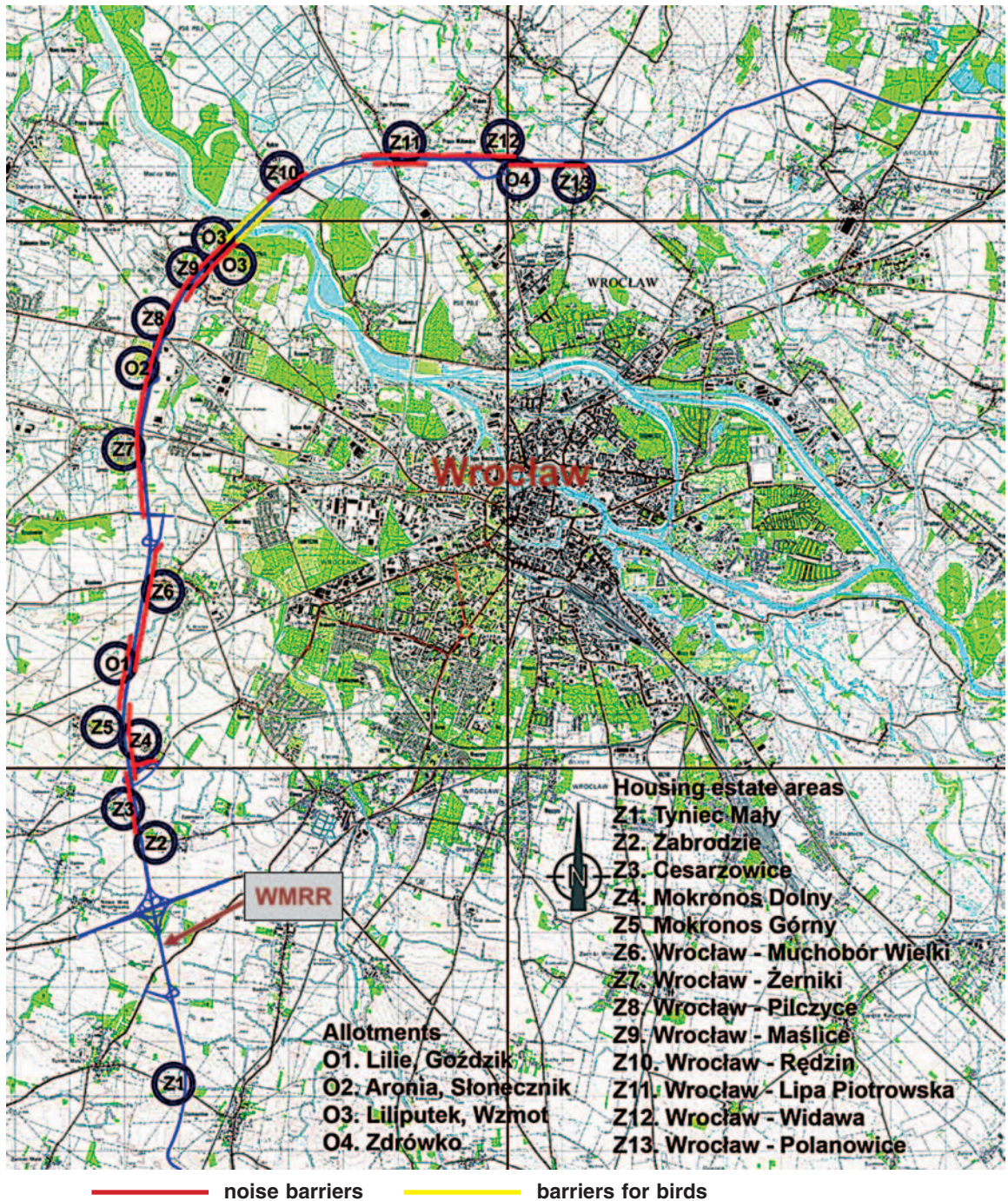
Figure 1. Location of Wrocław's motorway ring-road (WMRR). Notes. Z1–Z13—housing estates, O1–O4—allotments.
