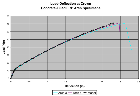
Figure 5. Arch Specimen Load-Vertical Deflection at Crown
