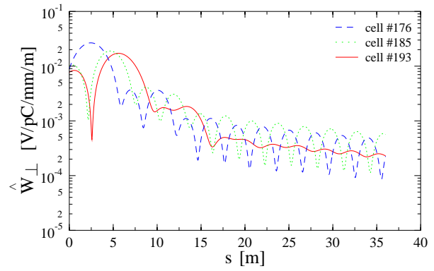
Figure 5: Wakefield envelope of transverse kicks at 11.4 GHz due to one misaligned cell.
