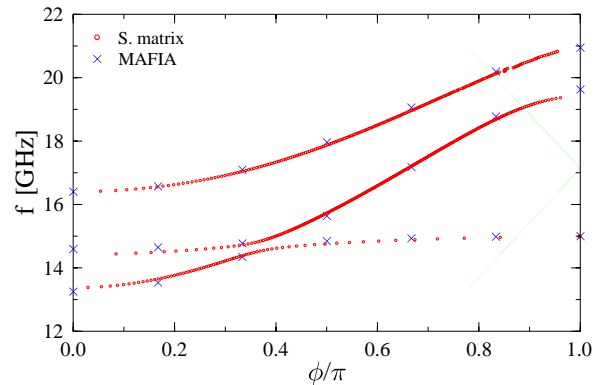
Figure 6: Dispersion curves for the geometry of cell 106 of DDS3, including 2 dipole and 1 manifold mode.
