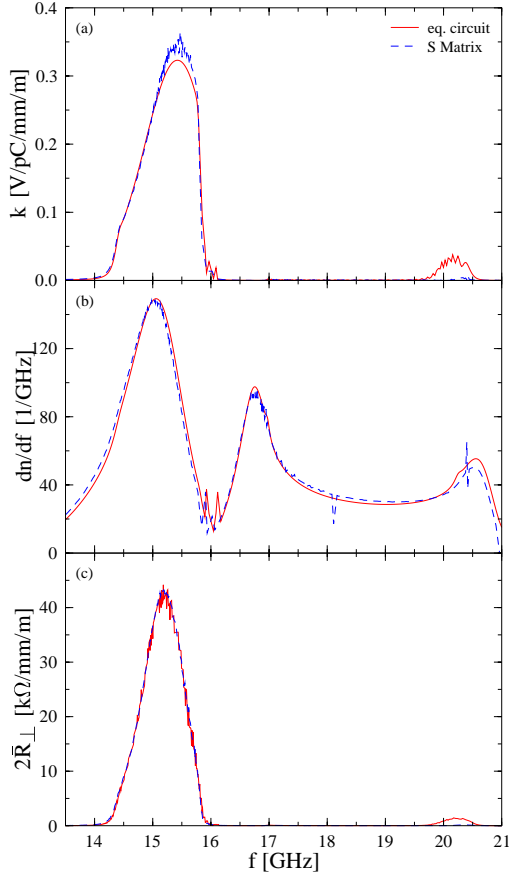
Figure 1: Comparison with the circuit model.
