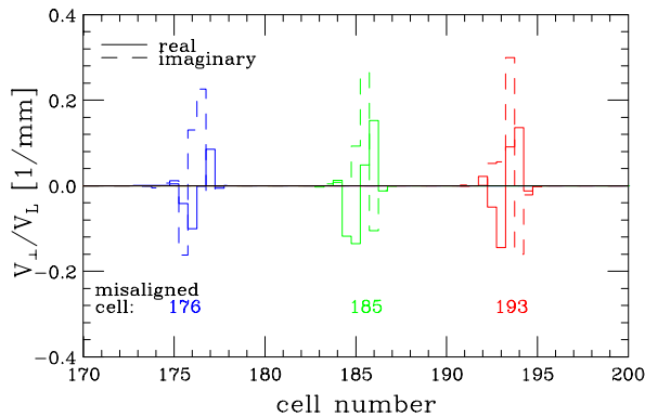
Figure 4: Real and imaginary parts of the ratio of transverse to longitudinal voltage, excited at 11.4 GHz by an on-axis beam, in a DT structure with one cell misaligned.
