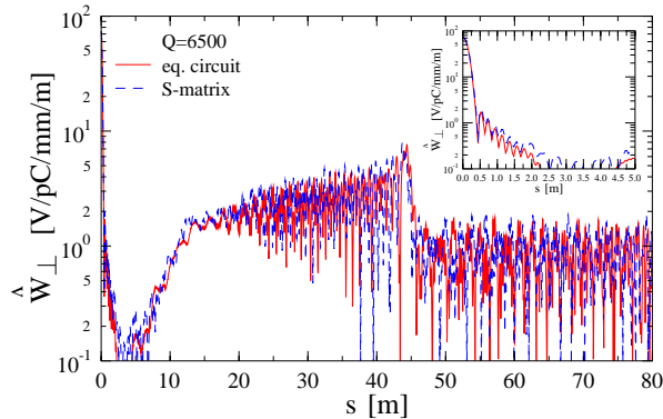
Figure 1: Comparison with the circuit model.
