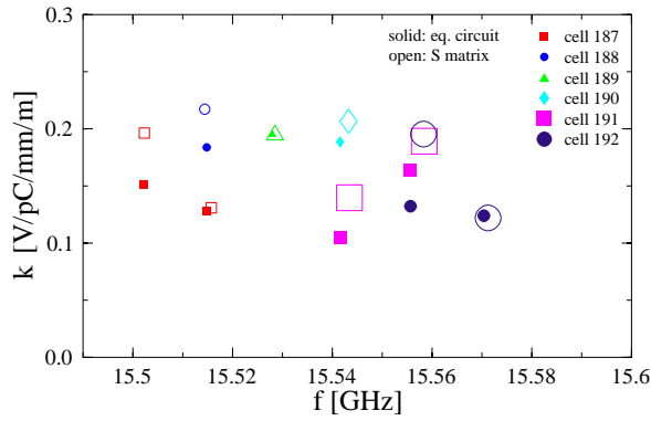
Figure 3: Largest kick factors for dipole modes near 15 GHz, in a DT structure with one cell misaligned.
