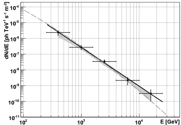
Fig. 2. Differential energy spectrum of the Crab Nebula. Black line: power law fit to the data, gray band: systematic uncertainties, dashed line: published data taken at low zenith angles [9].
