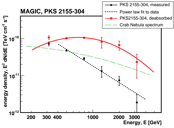
Fig. 5. Measured and intrinsic differential energy density of PKS 2155-304. The effect of the EBL is taken into account by using the recent model of Kneiske adopted by MAGIC [17]. The power law fit to the observed spectrum is given by the dotted line, while the curved fit to the intrinsic spectrum is shown by the solid line. The fitted peak position is located at E_{peak} = (672^{+104}_{-157}) GeV. For comparison the Crab Nebula spectrum is shown as the dashed line.
