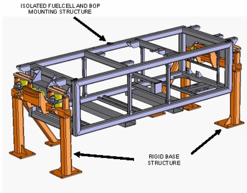
Fig. 7. All fuel cell stacks and balance of plant components mount to an isolated structure. The isolated structure provides protection during the harsh duty of the switcher locomotive.
