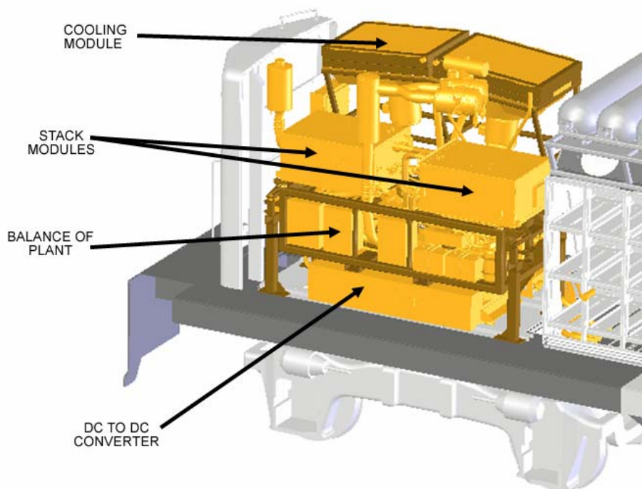
Fig. 5. Rear compartment layout. Systems were designed as bolt in modules, requiring minimal modifications to the locomotive platform. This allows for off line fabrication and testing of modules prior to vehicle installation.
