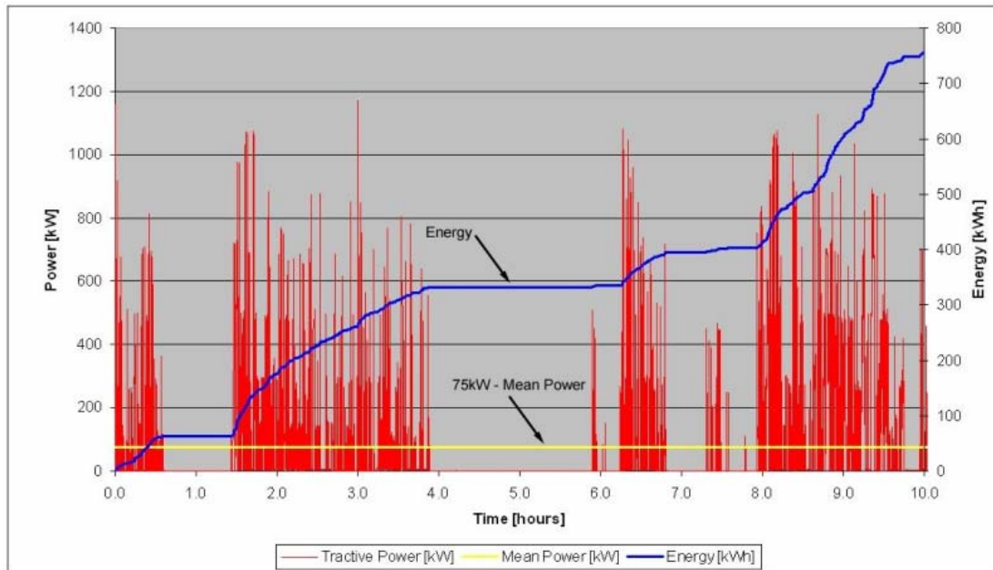
Fig. 2. Example switcher locomotive duty cycle. 75kW mean power is based on 20-h shift.
