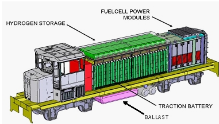
Fig. 6. Compressed hydrogen is stored in fourteen cylinders above the traction battery. A ballast weight will replace the diesel fuel tank to maintain tractive effort and center of gravity.
