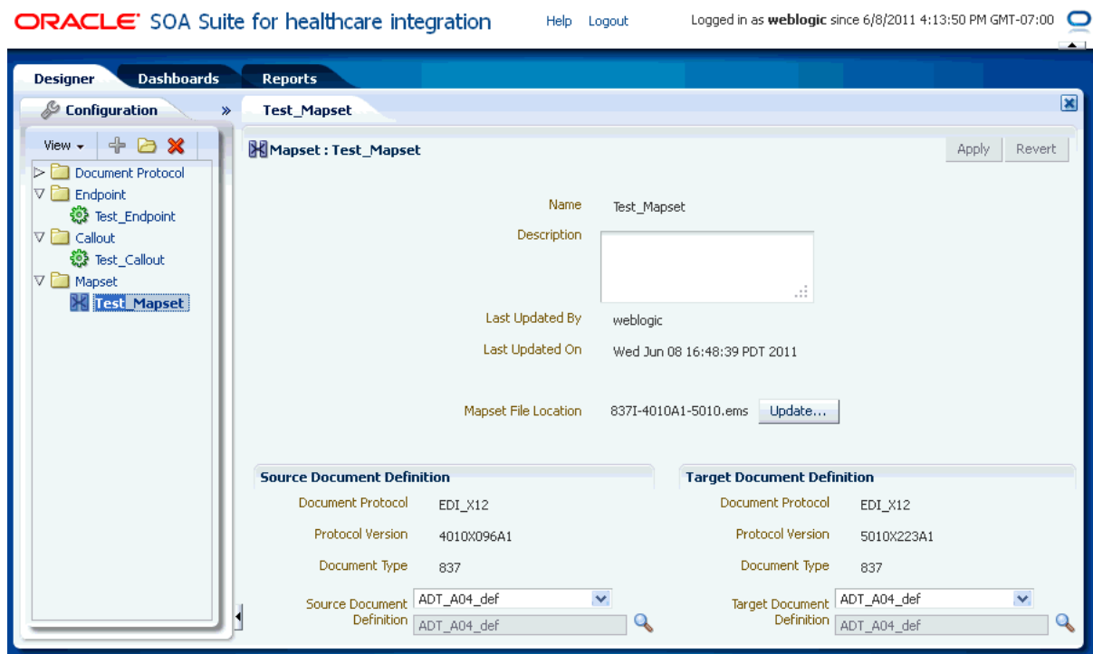
Figure 1–7 Sample Mapset
