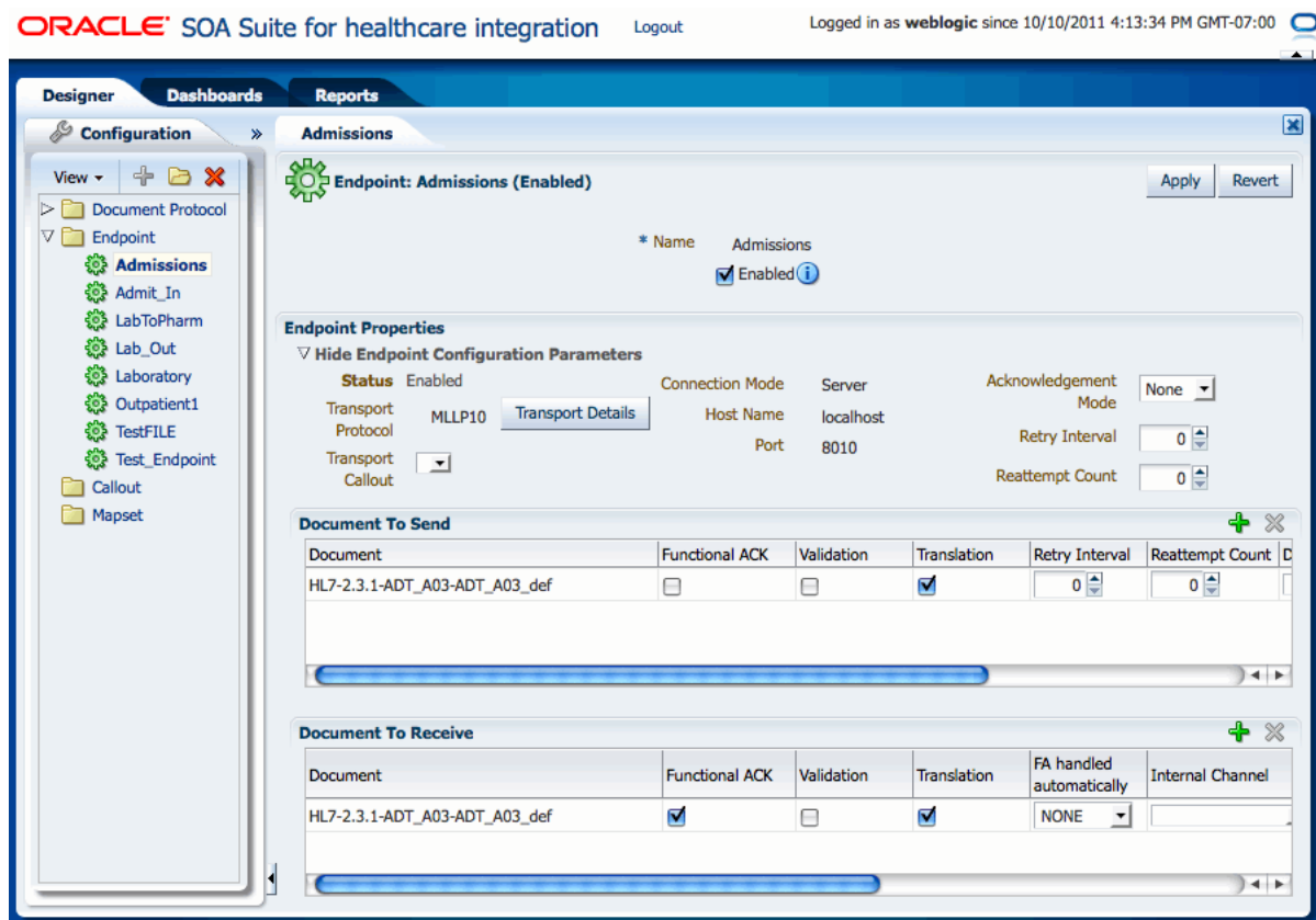
Figure 1–5 Sample Endpoint
