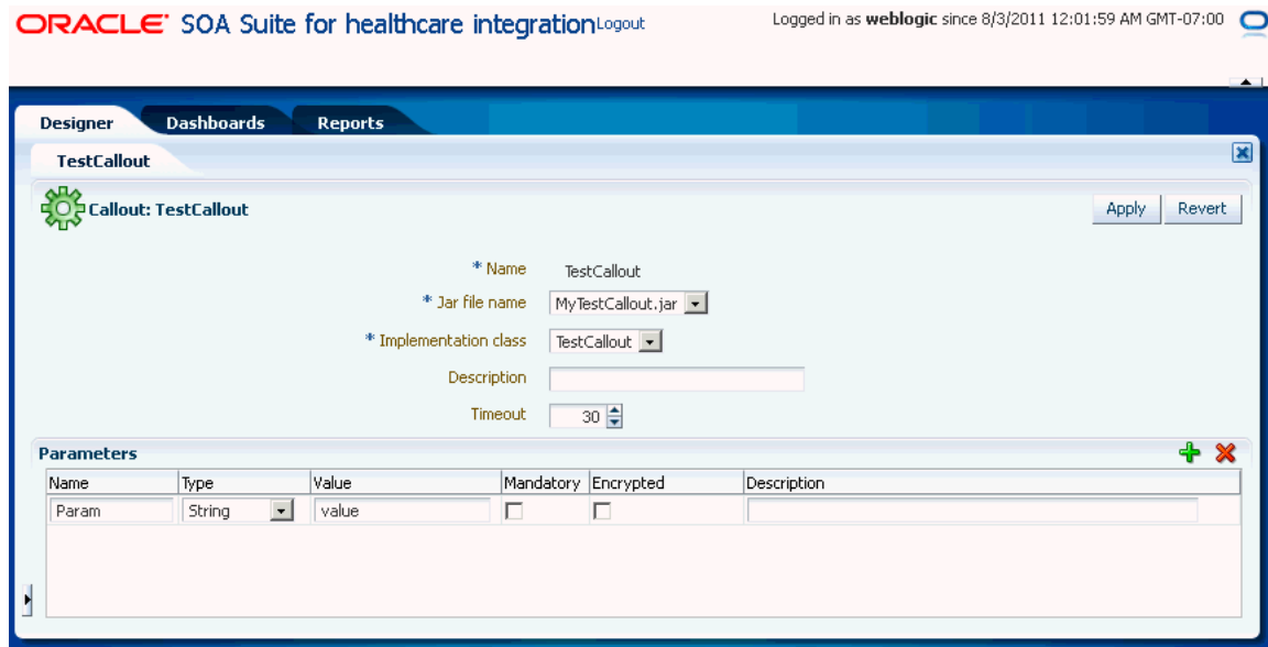
Figure 5–4 Configuring Callouts
