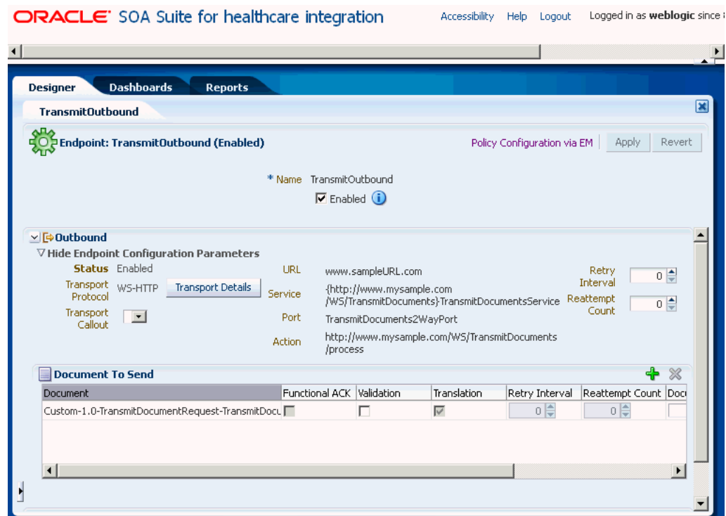
Figure 15–5 Configuring an Endpoint for Outbound Message Exchange
