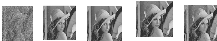
Figure 4. a) Noisy image with 80% Noise Density & PSNR of 5.98. Restriction results obtained for b) 'X1' with PSNR of 28.47 c) 'X3' with PSNR of 28.5 d) X4 with PSNR of 27.32 e) X4 with PSNR 26.26
