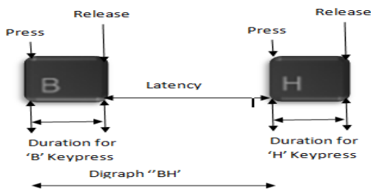
Fig 2 Duration, Latency and Digraph for the word “BH”
