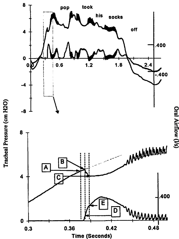
Figure 2. Method for measurement of the resistance of the lower airway ( R_{lw} ).
