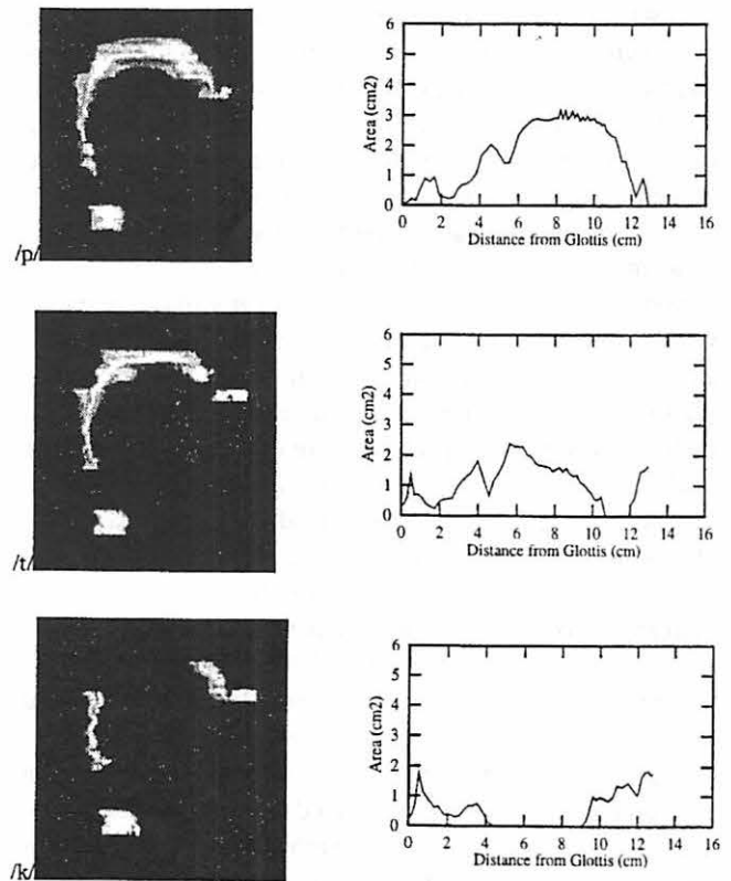
Figure 9. Surface rendered shapes and area functions for plosives (subject DJ).
