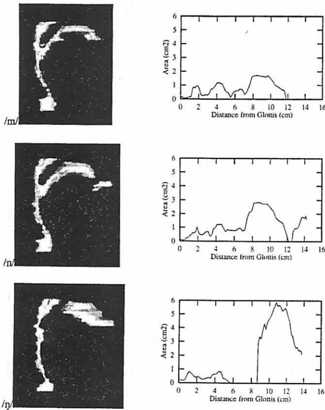
Figure 8. Surface rendered shapes and area functions for nasals (subject DJ).
