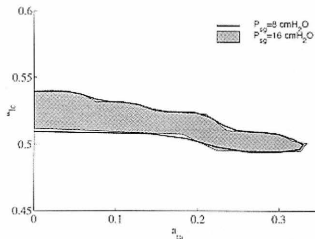
Figure 5. Zoomed-in adductory muscle activation plot (MAP) for higher level of cricothyroid activity ( a_{CT} = 0.6 ), (a) lung pressure = 8 cm H 2 O, (b) lung pressure = 16 cm H 2 O.
