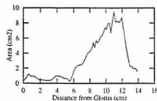
Figure 5. Surface rendered airways and “raw” area functions for /ʌ /, /ɑ/, and /ɔ/ (subject DJ).
