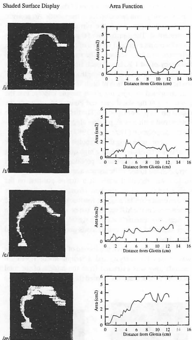
Figure 4. Surface rendered airways and "raw" area functions for /i/, /ɪ/, /ɛ/, and /æ/ (subject DJ).
