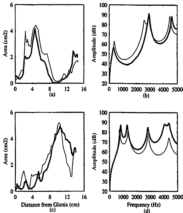
Figure 13. Comparison of /i/ and /ɑ/ acquired using MRI (thin line) and EBCT (thick line): a) area functions for /i/, b) frequency response functions for /i/, c) area functions for /ɑ/, d) frequency response functions for /ɑ/.
