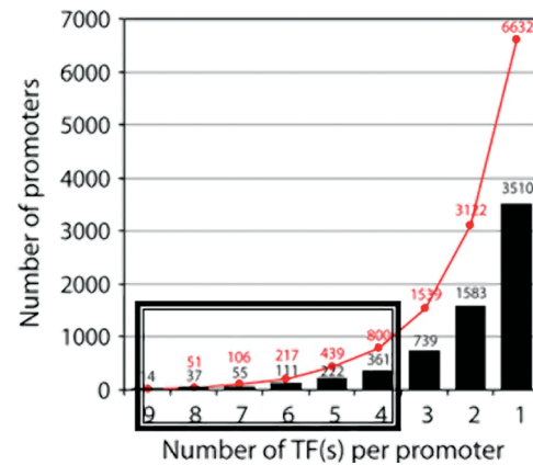
Figure 4. Distribution of numbers of factors bound to target proteins. Multifactor target genes (boxed) are defined as those promoters bound by more than four transcription factors among the nine tested. Approximately 800 target loci are represented in the multifactor category. (Modified from Kim et al. 2008 [© Elsevier].)
