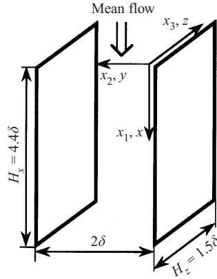
FIGURE 1. Calculation configuration.
