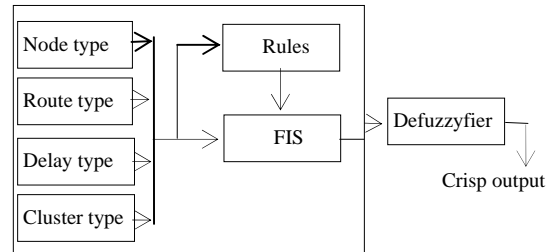
Fig. 7 Fuzzy Inference System (FIS)
