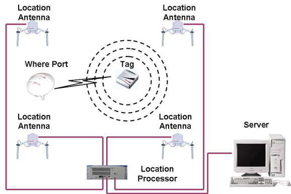
Fig. 11. WhereNet's Real Time Locating System
