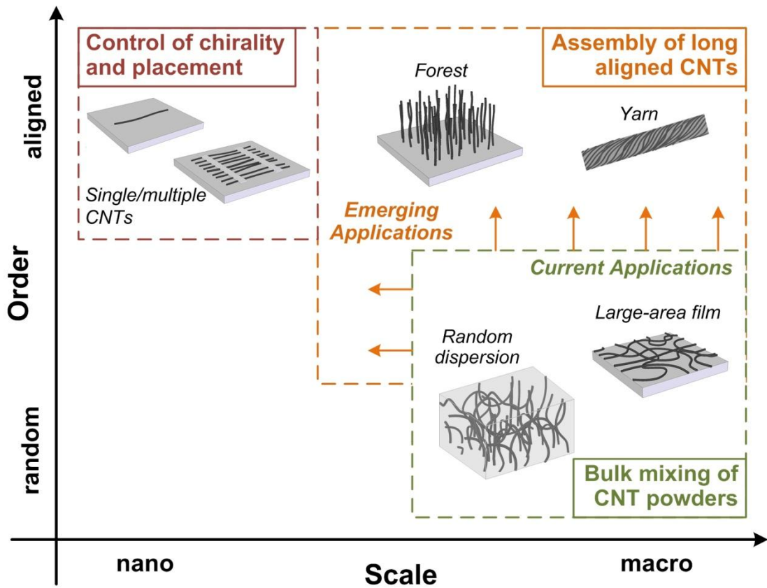
Figure S1: Emerging CNT applications rely on ordering of CNTs at hierarchical scales, moving from large-scale dispersions and films that are presently commercialized, to ordered macrostructures and nanoscale devices in the future.
