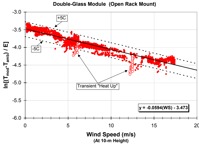
Fig. 8: Experimentally determined relationship for back surface temperature of a flat-plate module in an open-rack mounting configuration as a function of solar irradiance, ambient temperature and wind speed. A linear regression fit to the data provides the coefficients (a, b) for the thermal model.
