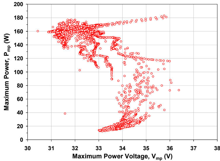
Fig. 1: Scatter plot of over 3300 performance measurements recorded on five different days in January in Albuquerque with both clear sky and cloudy/overcast operating conditions for a 165-W p mc-Si module.
