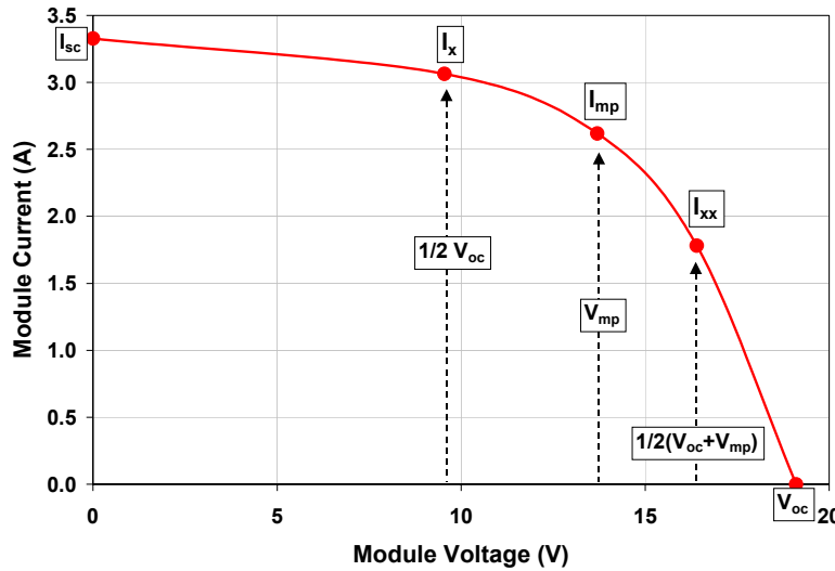
Fig. 2: Illustration of a module I-V curve showing the five points on the curve that are provided by the Sandia performance model.
