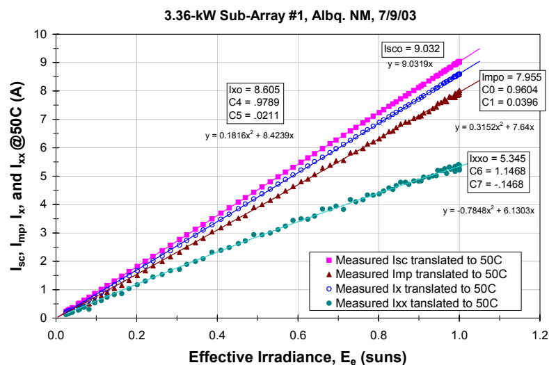
Fig. 9: Array current measurements recorded on a clear day for a 3.4-kWp array of c-Si modules in Albuquerque, New Mexico. The measured values were translated to a common temperature, 50^{\circ}\text{C} , before the regression analyses used to determine performance coefficients.
