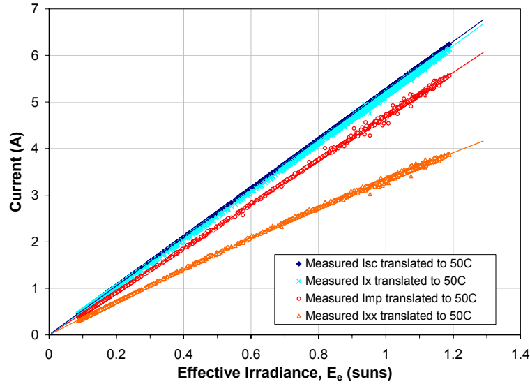
Fig. 4: Over 3300 measurements recorded on five different days with both clear sky and cloudy/overcast operating conditions for 165-W p mc-Si module. Measured values for currents were translated to a common temperature, 50°C, prior to regression analysis.
