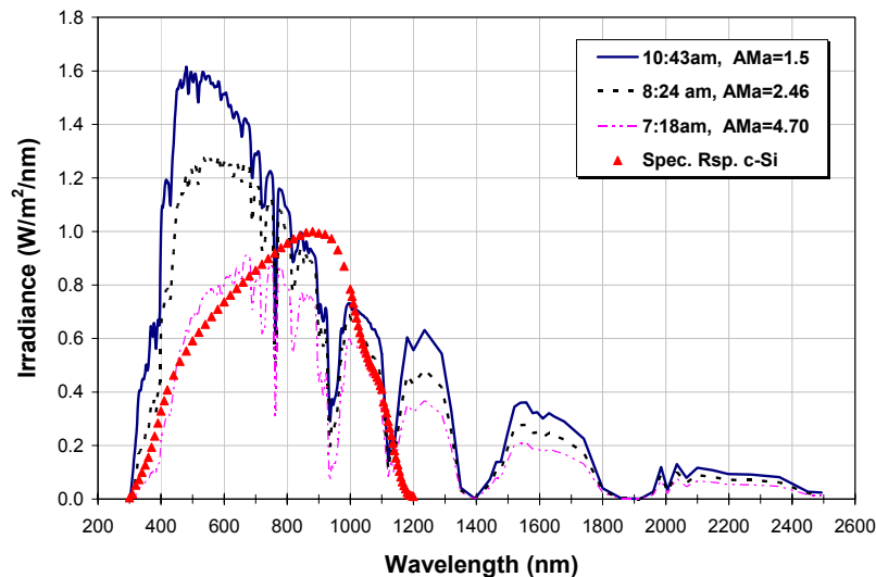
Fig. 5: Measured solar spectral irradiance on a clear day in Davis, CA, at different air mass conditions during the day, compared to the normalized spectral response of a typical silicon solar cell.
