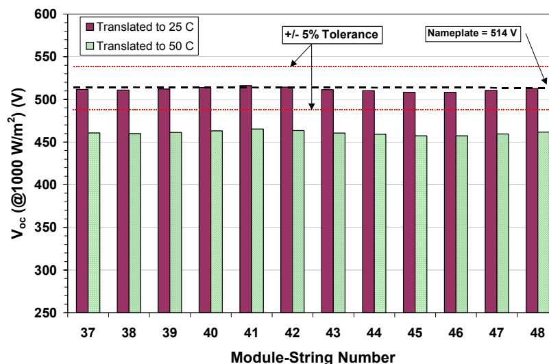
Fig. 17: Example of module-string V_{oc} measurements translated to the Standard Reporting Condition for comparison to expected nameplate value. Module-strings had twelve 150-W p c-Si modules in series. The translation to a 50°C temperature is also shown for comparison.
