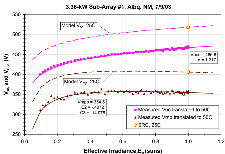
Fig. 10: Array voltage measurements recorded on a clear day for a 3.4-kWp array of c-Si modules in Albuquerque, New Mexico. The measured values were translated to a common temperature, 50^{\circ}\text{C} , before the regression analyses used to determine performance coefficients. The reference values at the ASTM Standard Reporting Condition are also shown.
