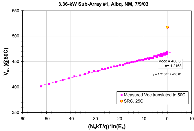
Fig. 11: Regression analysis used to determine performance coefficients for array open-circuit voltage. The measured V_{oc} values were translated to a common temperature, 50°C, before the regression analysis. The reference V_{oc} value at the ASTM Standard Reporting Condition is also shown. N_s = 864 for the array.
