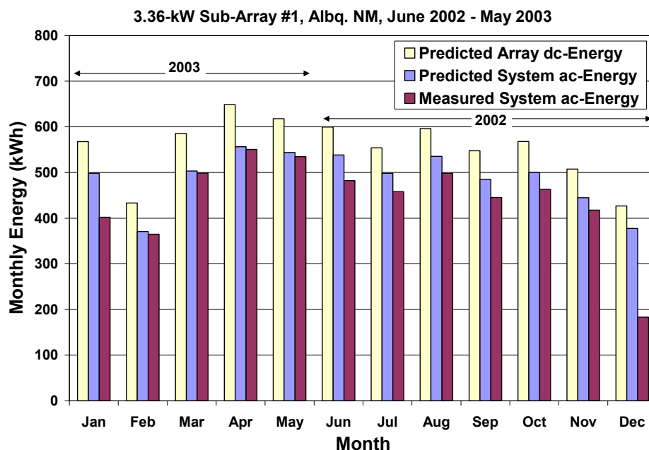
Fig. 14: Comparison of predicted and measured monthly energy production for a 3.36-kW grid-connected photovoltaic system in Albuquerque, NM. Chart shows predicted dc-energy available from the array, as well as the predicted and measured ac-energy provided by the system.
