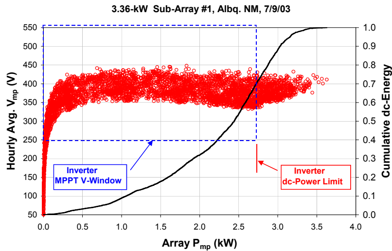
Fig. 15: Scatter chart of calculated hourly-average performance values for 3.36-kW array in Albuquerque, NM, over a one year period. Superimposed are the voltage and power constraints for the inverter used with the system. The fraction of the cumulative annual energy available from the array is also shown as a function of the array power level.
