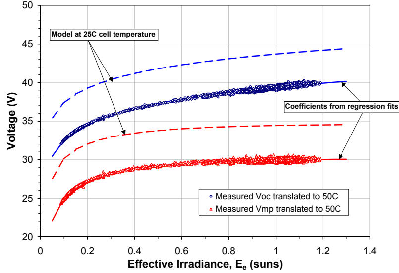
Fig. 3: Over 3300 measurements recorded on five different days with both clear sky and cloudy/overcast operating conditions for 165-W p mc-Si module. Measured values for V_{oc} and V_{mp} were translated to a common temperature, 50°C, prior to regression analysis. Performance model provides the predicted curves at 25°C.
