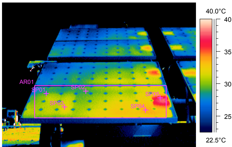
Fig. 18: Thermal infrared (IR) image of several modules in an array illustrating the spatial variation in module temperature often present due to wind cooling, mounting structures, junction boxes, etc.
