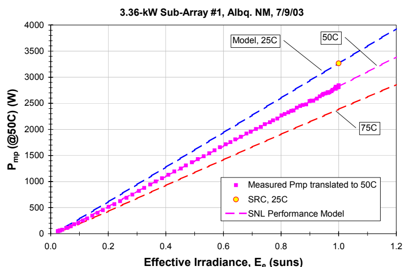
Fig. 13: Demonstration of performance model for array maximum power at three operating temperatures as a function of effective irradiance. Field measurements translated to 50°C are shown for comparison. The reference P_{mp} value at the ASTM Standard Reporting Condition is also shown.
