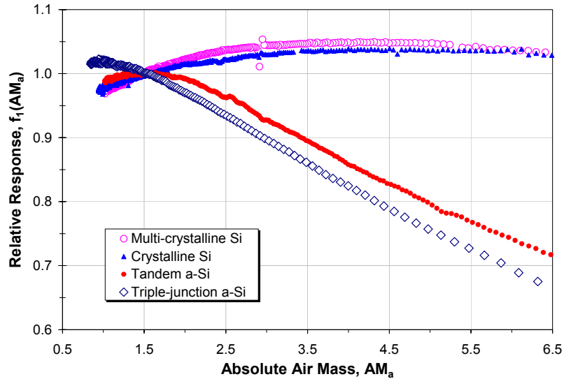
Fig. 6: Typical empirical relationship illustrating the influence of solar spectral variation on module short-circuit current, relative to the AM_a=1.5 reference condition. Results were measured at Sandia National Laboratories for a variety of commercial modules.
