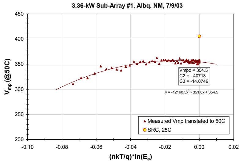
Fig. 12: Regression analysis used to determine performance coefficients for array maximum-power voltage. The measured V_{mp} values were translated to a common temperature, 50°C, prior to the regression analysis. The reference V_{mp} value at the ASTM Standard Reporting Condition is also shown. N_s = 864 for the array. Trend line coefficients must be divided by N_s to obtain C_2 , C_3 coefficients.
