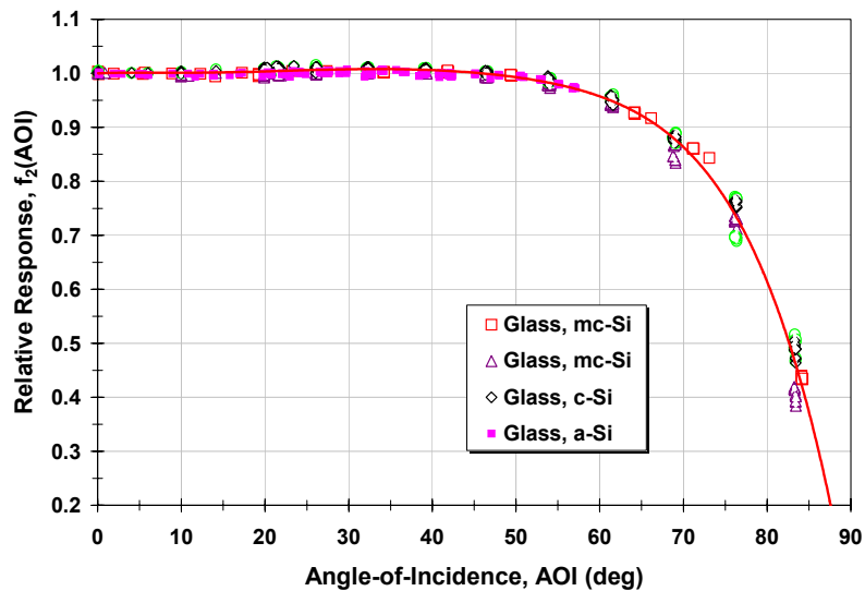
Fig. 7: Typical empirical relationship illustrating the influence (optical loss) of solar angle-of-incidence on a module's short-circuit-current. Results were measured at Sandia National Laboratories for four different module manufacturers. The effect is dominated by the reflectance characteristics of the glass surface.
