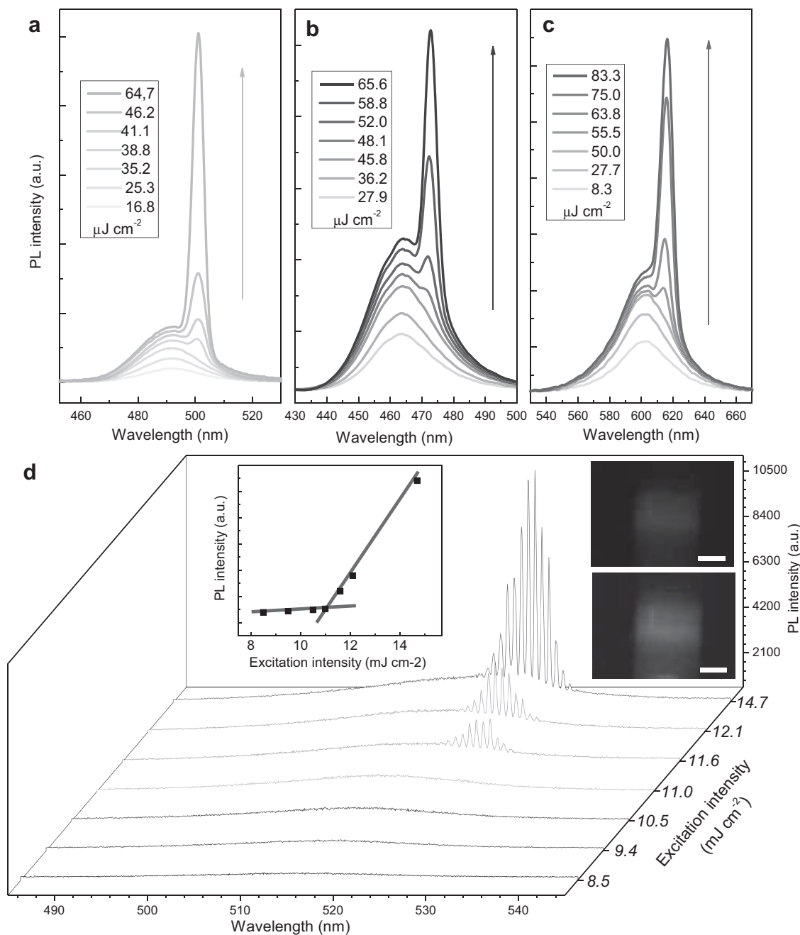
Figure 6. a) Stimulated emission from small sized-CsPbBr 3 IPQDs, showing blue-shifted stimulated emission wavelength. b) Blue stimulated emission from CsPb(Br/Cl) 3 IPQDs. c) Red stimulated emission from CsPb(I/Br) 3 IPQDs. d) Pump intensity-dependent PL spectra from CsPbBr 3 IPQDs with edge length of ≈9 nm infiltrated into a capillary tube with inner diameter of ≈50 μm. The left inset displays the spectrally integrated PL intensity over the lasing peaks with respect to pump intensity. The optical images of the IPQDs infiltrated capillary tube below (upper image) and above (lower image) the lasing threshold are presented as the right insets. Scale bar is 20 μm.
