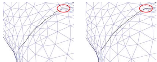
Figure 7: Low-resolution model with suggestive contours found using linear ( left ) or cubic Hermite ( right ) interpolation. The latter approach uses not only the value but also the gradient of \kappa_r at each vertex to improve the estimated locations of \kappa_r = 0 .
