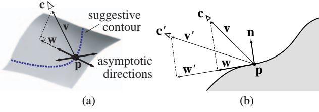
Figure 2: (a) \mathbf{w} is the projection of the view direction \mathbf{v} onto the tangent plane. At a suggestive contour, \mathbf{w} points in one of the asymptotic directions of the surface—directions in which the curvature is zero. (b) Suggestive contours do not move when the camera motion is in the radial plane (from \mathbf{c} to \mathbf{c}' ) because the direction of \mathbf{w} does not change (only the length of \mathbf{w}' is different, not its direction)
