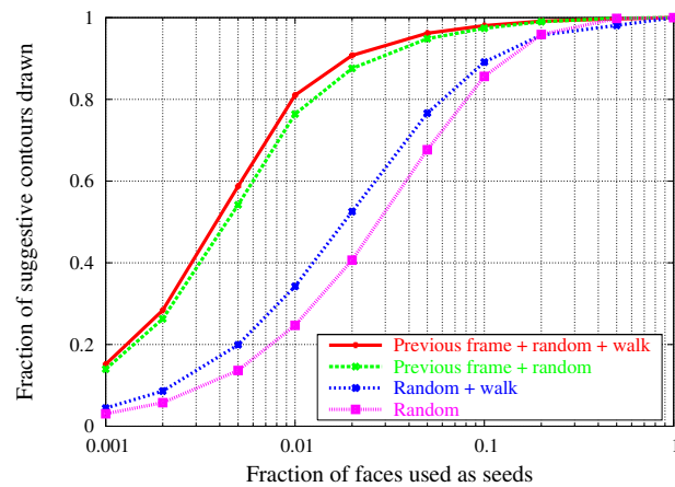
Figure 6: Randomized techniques can reduce the number of faces that need to be tested for suggestive contours.
