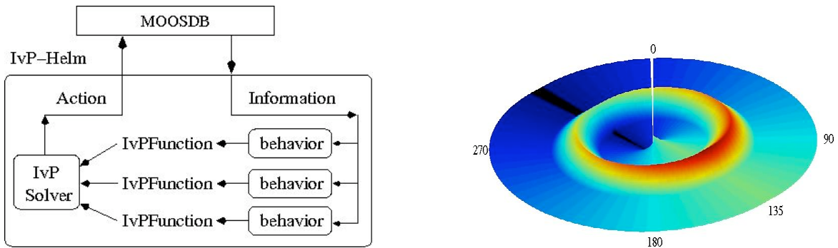
Figure 3: The IvP Helm is a MOOS module that implements a behavior-based architecture using multi-objective optimization for behavior coordination. On the left is the basic structure and flow of control and information during a single control loop iteration. On the right an objective function produce by a simple waypoint-following behavior is shown. The plot is shown in polar
