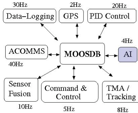
Figure 2: A MOOS community consists of a number of (typically Linux) processes running separately, perhaps on different machines, communicating via TCP/IP through a single database process (MOOSDB) in a publish-subscribe framework. MOOS also provides basic functionality for requesting the frequency in which a process executes its primary routine.
