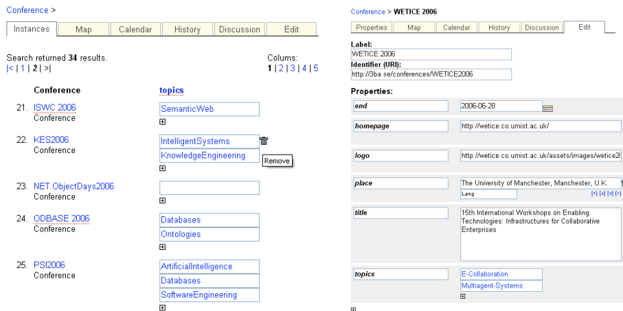
Figure 4. Editing of a property's values at many instances at once (left). Dynamically generated form combining different widgets based on an OWL class definition (right).
