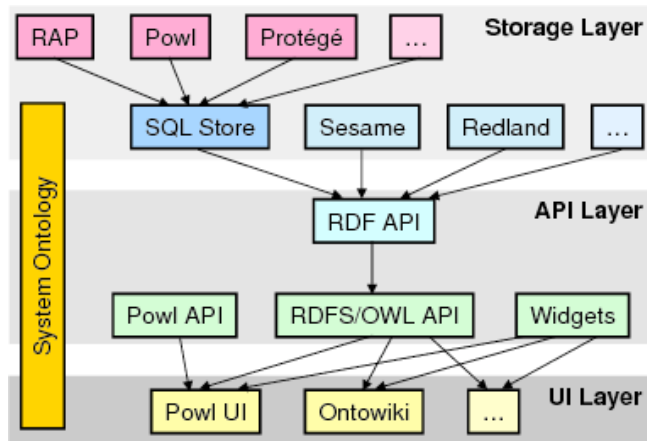
Figure 7. Architecture of Powl and OntoWiki.
