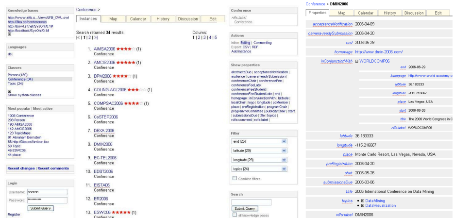
Figure 1. List view (left) and view of an individual instance with expanded inline reference view (right).
