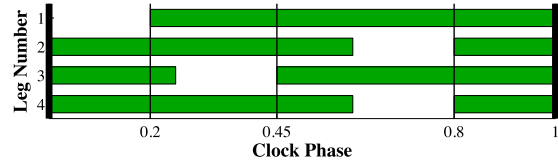
Fig. 6: The relative timing of stance (shaded) and recirculation for the climbing. The front legs (1 and 3) recirculate individually, with back legs moving together. At high speed, the robot repeats this gait at 1.75 Hz, once every 0.57 seconds.
