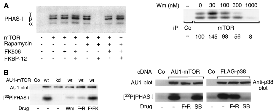
Fig. 2. Phosphorylation of PHAS-I by immunopurified mTOR. (A) Rat brain extracts were immunoprecipitated with anti-mTOR (+) or with nonimmune rabbit immunoglobulin G (-). Immune complex kinase reactions were done with recombinant PHAS-I as the substrate (23). The kinase reaction products were separated by SDS-PAGE, and 32 P-labeled PHAS-I was detected by autoradiography. In the right panel, rat brain extracts were immunoprecipitated (IP) with rabbit immunoglobulin G (Co) or with anti-mTOR, and immune complex kinase reactions were done as described above. The numbers below the sample lanes represent [ 32 P]phosphate incorporated into PHAS-I, as a percentage of that in the non-wortmannin (Wm)-treated control. (B) AU1-tagged mTOR-wt and mTOR-kd (left panel) or FLAG-tagged p38 (right panel) were immunoprecipitated from transfected K562 cells (25). Control transfections (Co) were performed with pcDNA3 only. The immunoprecipitates were treated with GST-FKBP12 plus rapamycin (F•R) or FK506 (F•FK), or 5 \mu M SB203508 (SB), and immune complex kinase assays were performed with PHAS-I as the substrate. 32 P-labeled PHAS-I (bottom panels) was detected by autoradiography. The immunoprecipitated mTOR and p38 were visualized by immunoblotting with mAb AU1 and anti-p38, respectively (top panels). (C) Phosphoamino acid analysis of PHAS-I phosphorylated in vitro by recombinant mTOR. Two-dimensional separation of phosphoserine (S), phosphothreonine (T), and phosphotyrosine (Y) was done as described (26).
