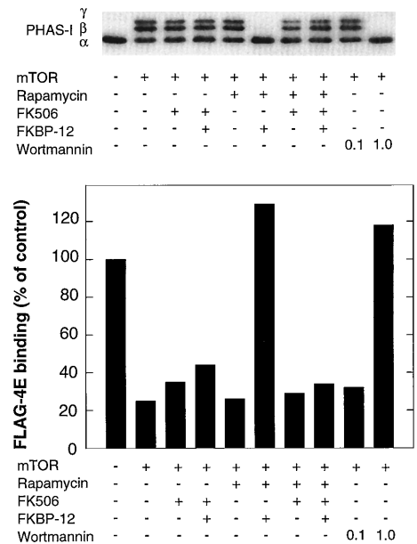
Fig. 3. The eIF-4E-binding activity of phosphorylated PHAS-I. Nonimmune rabbit immunoglobulin G (-) or anti-mTOR (+) immunoprecipitates from rat brain were incubated with the indicated agents, and immune complex kinase assays were done with recombinant PHAS-I and nonradioactive ATP (23). The concentrations of wortmannin are given in micromolar. (Top) Reaction products were separated by SDS-PAGE, and phosphorylated forms of PHAS-I were detected by immunoblotting. (Bottom) The eIF-4E-binding activity of PHAS-I was determined by Far-Western analysis with 32 P-labeled FLAG-eIF-4E as a probe (6). Radioactivity bound to PHAS-I was quantitated and normalized to the mock-phosphorylated control.
