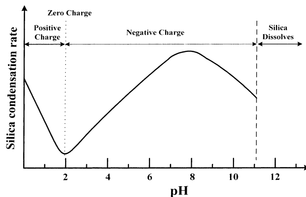
FIGURE 1. Effects of pH value on the silica condensation rate and silicas surface charge properties.
