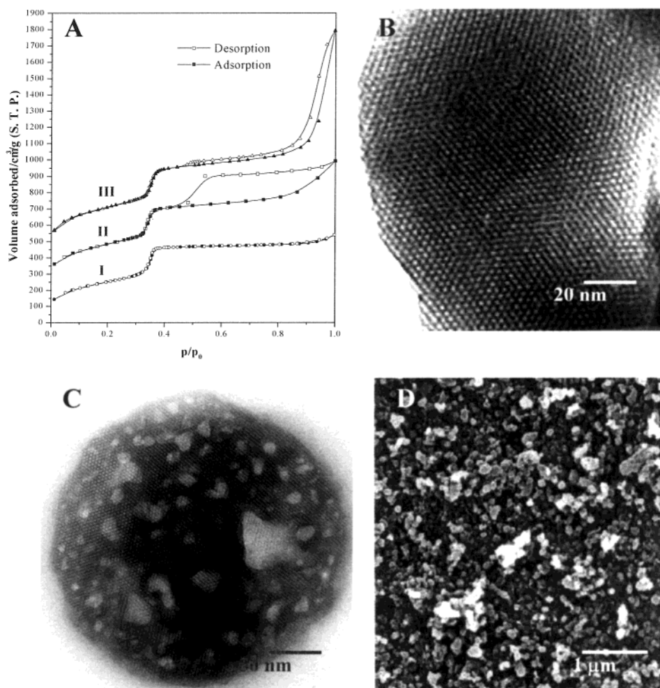
FIGURE 7. (A) N 2 adsorption–desorption isotherms of the mesoporous silica and aluminosilicates samples obtained from C 16 TMAB–aluminosilicate–H 2 O systems by a delayed neutralization process. Sample I is a mesoporous silica (Si/Al = ∞) with microparticle form; sample II is a mesoporous aluminosilicate (Si/Al = 37) with TWT hierarchical structure, and sample III is a mesoporous aluminosilicate (Si/Al = 37) in the fine particulate form. (B) TEM micrograph of sample I. (C) Microtome TEM micrograph of the sample II. (D) SEM micrograph of sample III.
