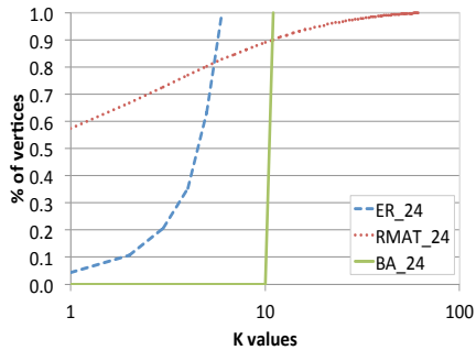
Figure 3: Cumulative K value distribution for synthetic graphs.
