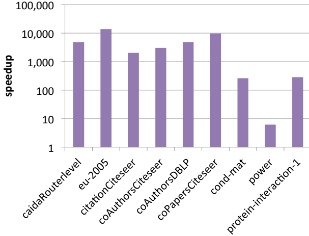
Figure 9: Subcore algorithm speedups for real datasets when compared to the baseline. Our incremental algorithm runs up to 14,000× faster than the non-incremental algorithm.
