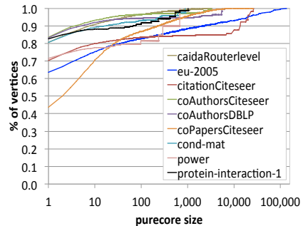
Figure 6: Cumulative purecore size distribution for real-world graphs.
