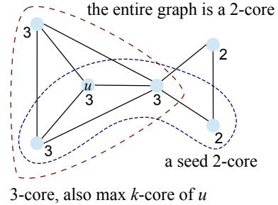
Figure 1: Illustration of k -core concepts.
