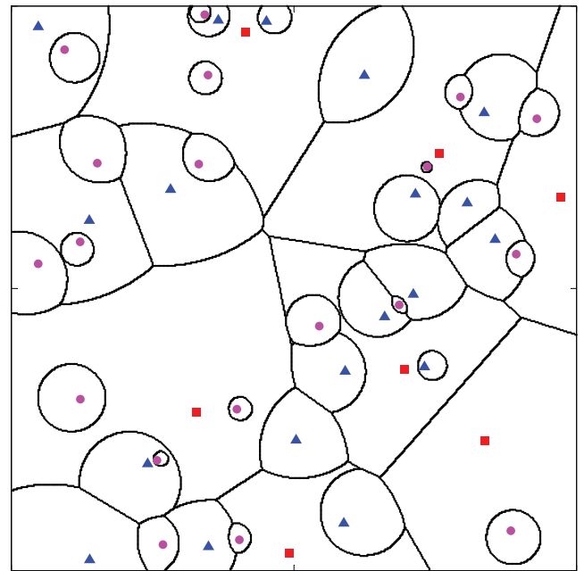
Fig. 5. Biased Cell Association in a 3-tier Heterogenous Network. Picos and femtos have a 10 dB bias.
