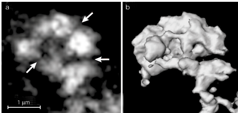
Supplementary figure 1 | 3q-chromosome-arm domain exemplifies a complex sponge-like chromosome territory structure. a | Light optical nuclear section showing a painted 3q-arm domain from a neuroblastoma HD-N-16 cell (courtesy of Irina Solovei and Dirk Kienle) (compare with another section from the same arm domain in figure 19b from REF. 29). Arrows indicate sites of channel-like invaginations that lead from the arm-domain periphery into the interior and throughout the entire arm domain. b | Three-dimensional reconstruction of the 3q-arm domain shows its complex surface with openings of invagination/interchromatin-compartment (IC) channels. The accessibility of these IC channels is shown by the fact that double-minute chromosomes were noted in the domain interior (not shown, compare with figure 19 in REF. 19). Double minute — small chromosomal fragments frequently seen in cancer cells.
