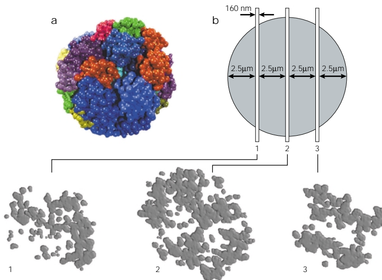
Supplementary figure 2 | The spherical ~1-Mb chromatin-domain model. a | This model of a male diploid human cell nucleus shows 46 independently distributed chromosome territories (CTs) visualized using 24 pseudocolours (courtesy of Gregor Kreth) 91 . (Visualization was done using Persistence of Vision (TM) Ray-Tracer Pov-Ray ) b | Three virtual nuclear sections were generated from the model nucleus at the indicated sites after digitization of the data stack. The resulting, grey-coloured 'low resolution' ultrastructural sections show an interchromatin compartment space of variable width expanding between the spherical chromatin domains. The borders of the individual CTs, however, can no longer be distinguished. This provides a reason why CTs have been missed by electron microscopists.
