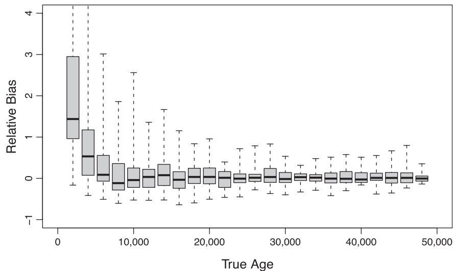
FIG. 1. Relative bias in posterior mean leaf-age estimates from 960 leave-one-out analyses of synthetic data sets with varying true leaf-ages. For true ages sufficiently distinct from zero, the posterior mean estimator is unbiased.
