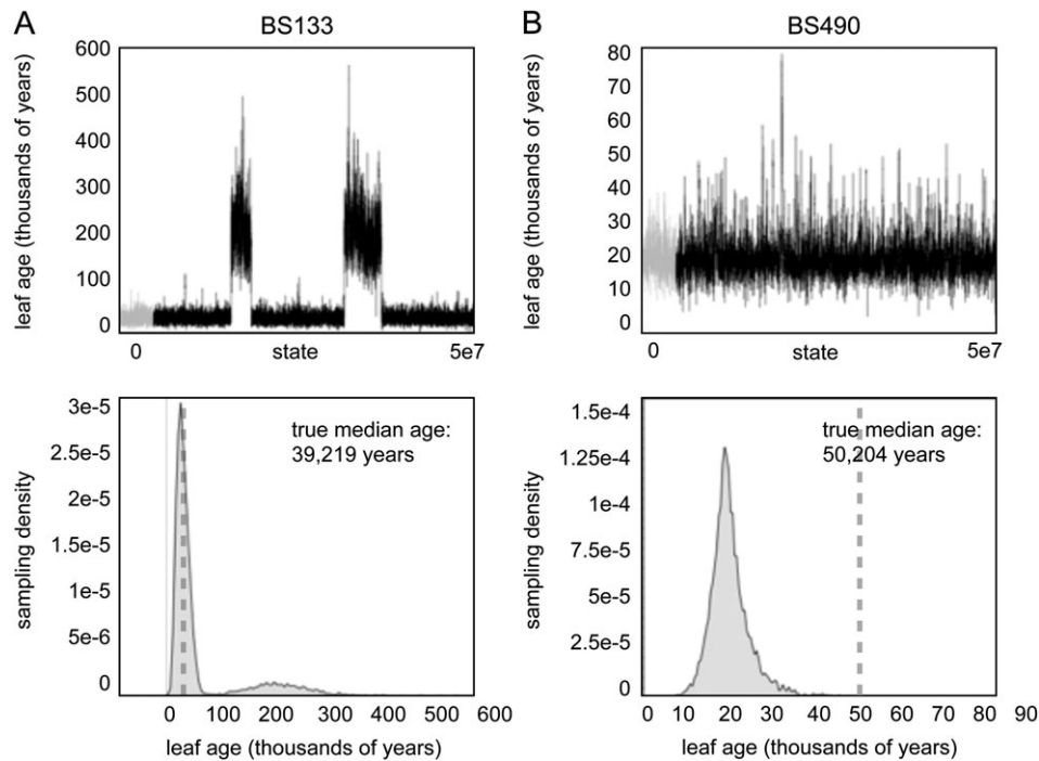
Fig. 3. Examples of two different leave-one-out analyses for which the true age was not recovered within the 95% HPDs of the leaf-age estimates. In (A), the analysis identifies two similarly likely leaf-ages, whereas in B the analysis identifies a single, precise estimate that does not coincide with the radiocarbon date of the specimen from which the sequence was isolated. By evaluating the trace files from each leaf-age estimate, it is possible to identify potentially erroneous sequences and to devise an appropriate strategy to authenticate these sequences.
