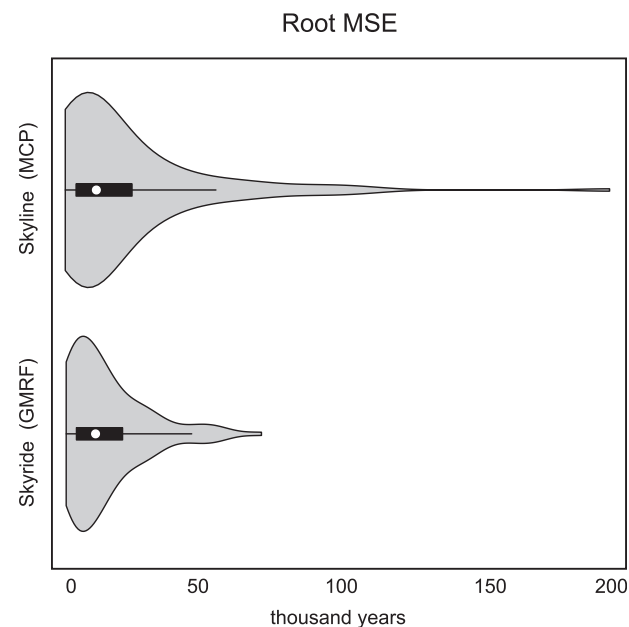
Fig. 2. Empirical distributions of rMSE when estimating leaf-dates under flexible coalescent models based on a multiple change-point (MCP) process and GMRF.
