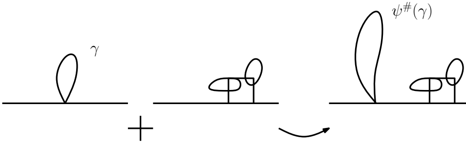
Figure 14: Construction of \mu_A (sketch)
