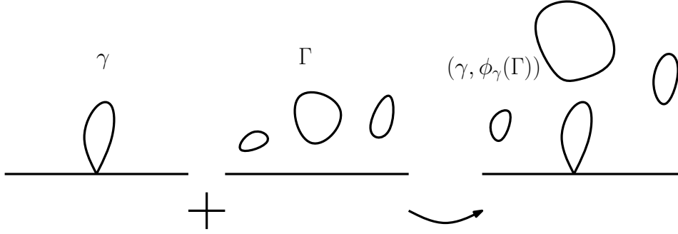
Figure 16: Construction of (\bar{\gamma}, \bar{\Gamma}) (sketch)
