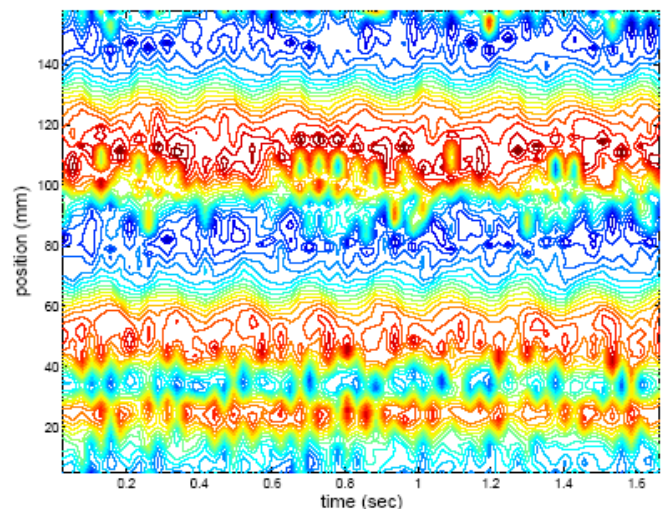
Fig. 11 Contours of axial velocity profile at Ta = 584
