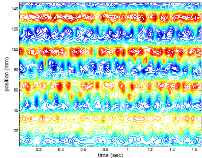
Fig. 3 Contours of axial velocity profile at Ta = 529
