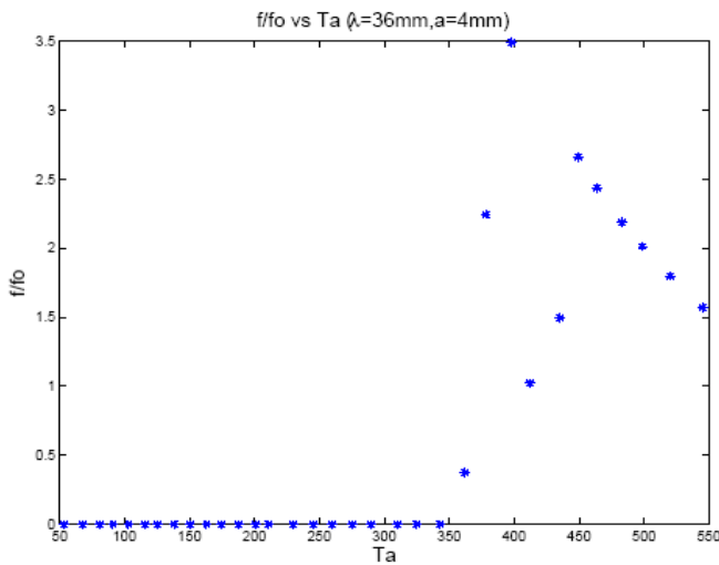
Fig. 1 Evolution of the frequency ratio ( f/f_o ) vs. Ta case C_1
