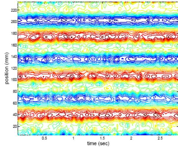
Fig. 7 Contours of axial velocity profile at Ta = 83
