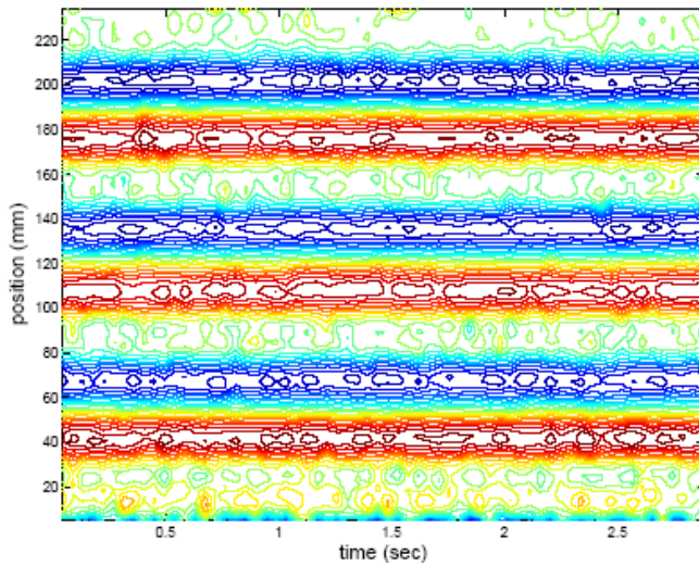
Fig. 8 Contours of axial velocity profile at Ta = 77
