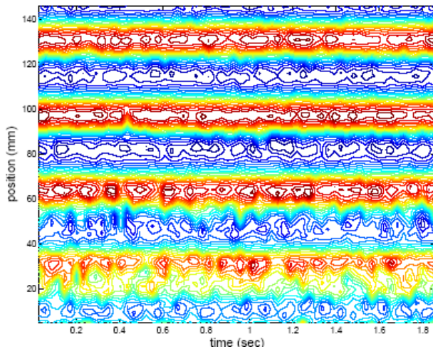
Fig. 5 Contours of axial velocity profile at Ta = 377
