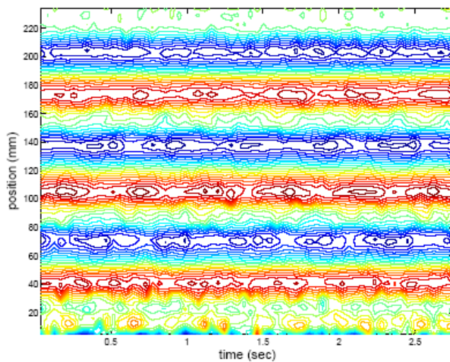
Fig. 9 Contours of axial velocity profile at Ta = 356
