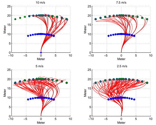
Figure 5: An example of whole set of trajectories at four speeds for a given initial steering
