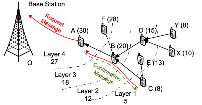
Fig. 2. Greedy helper discovery protocol and relay routing protocol. The numbers in parenthesis are the average 3G rates for each node. The dashed line indicates the ad-hoc neighborhood. The straight solid line is the ad-hoc path with the arrow pointing to the helper. For relay routing protocol, dashed-dotted lines represent the coverage area of each layer. The physical transmission rates for layers 4, 3, 2, and 1 are 27, 18, 12, and 5.
