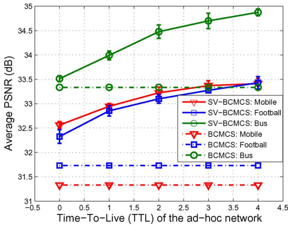
Fig. 6. Impact of TTL on the average PSNR.
