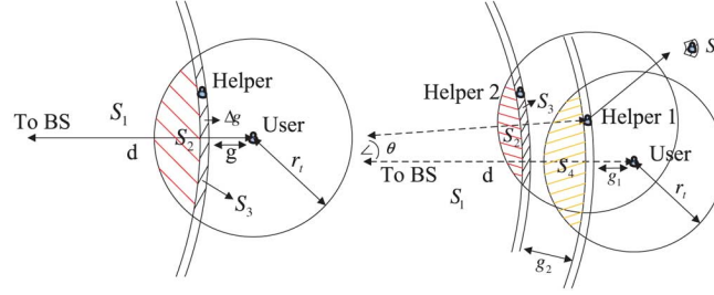
Fig. 3. (Left) One-hop and (right) two-hop ad-hoc relay analysis for an arbitrary user.
