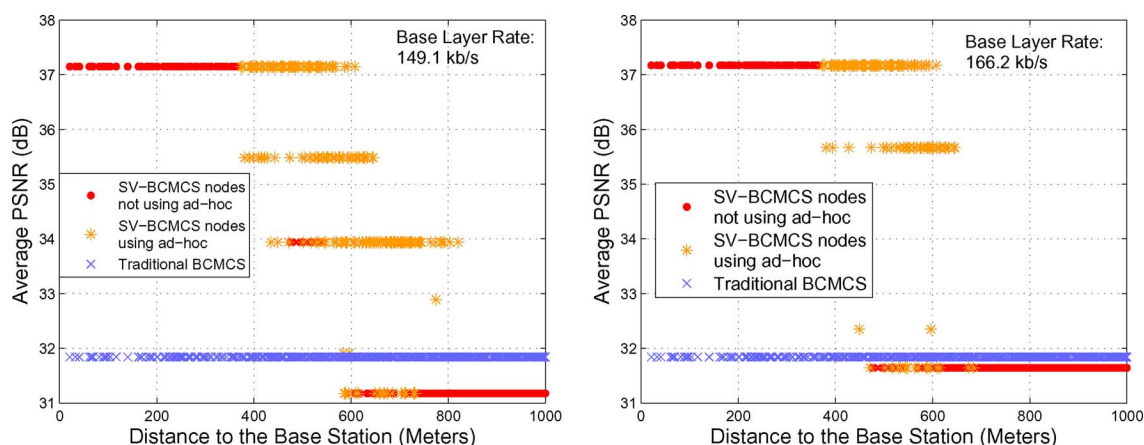
Fig. 9. Tradeoffs of the base layer rate and the overall performance in SV-BCMCS. Optimal resource allocation significantly improves the system-wide video rate at the price of a small quality decrease for nodes close to the boundary; ad-hoc relays further increase the video quality for all users. Almost all users achieve a higher video quality than in the traditional BCMCS.
