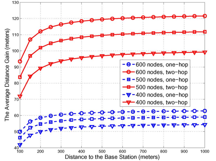
Fig. 4. One-hop and two-hop distance gain for nodes with different distance to the base station.
