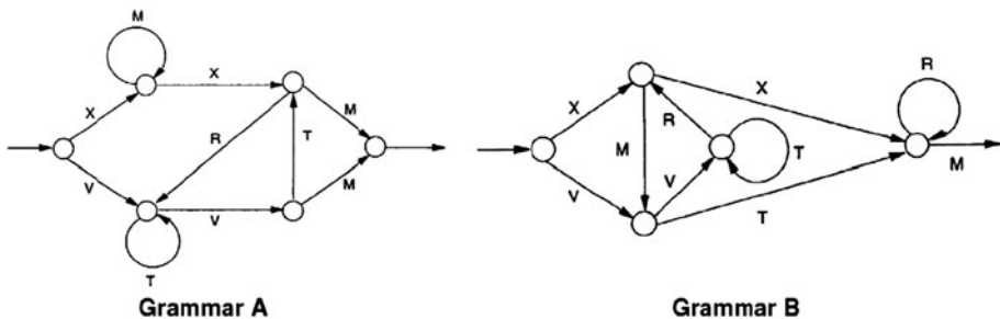
Fig. 1 The two finite state grammars used to generate the strings (taken from Reber 1967)
