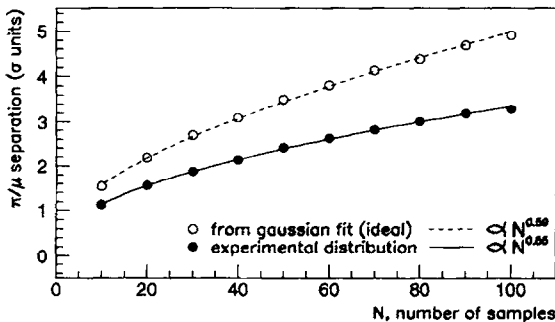
Fig. 15. \pi/\mu separation from a cluster counting measurement (full line) as a function of the track sampling. For comparison the ideal cluster counting separation is indicated (broken line).
