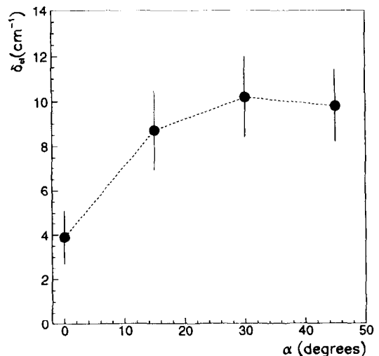
Fig. 11. Clusters density, \delta_{cl} , as a function of the angle \alpha between the track and the normal to the tube for a 25 \mu m wire diameter. The gas mixture used is 95%He 5% i C 4 H 10 , the high voltage on the sense wire is 1550 V and the beam momentum is 200 MeV/c.
