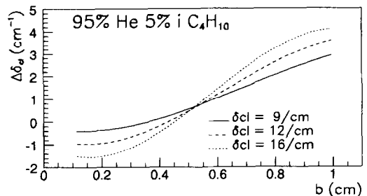
Fig. 7. Difference between the number of counted clusters according to the described algorithm and the generated number of clusters per unit length as a function of the impact parameter for different cluster density.
