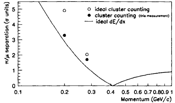
Fig. 16. \pi/\mu separation as a function of the particle momentum. The solid line is an empirical extrapolation from existing data.
