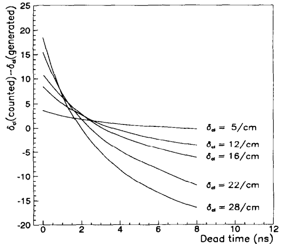
Fig. 6. Difference between counted and generated clusters as a function of the simulated dead time \tau . Longitudinal diffusion proper of a 90%He 10%iC 4 H 10 mixture.
