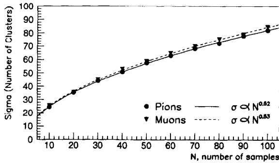
Fig. 14. Cluster counting resolution as a function of the track sampling, for pions and muons.
