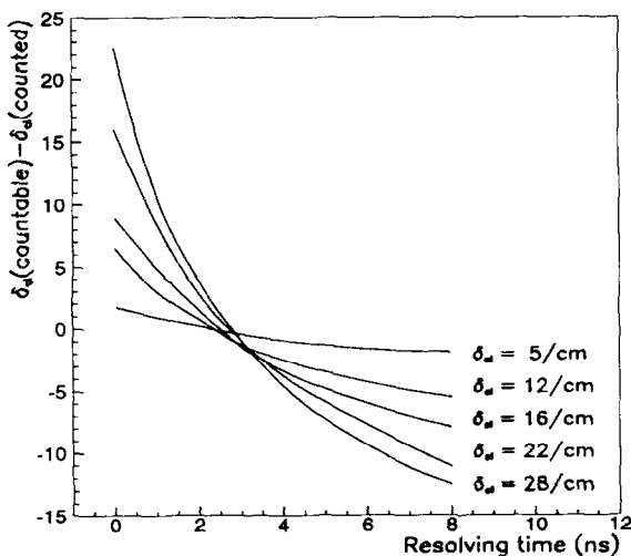
Fig. 9. Difference between the number of clusters which can be detected when a given dead time is simulated and the number of clusters counted by the algorithm for different primary ionization densities. The algorithm resolution is assumed to be equal to the simulated dead time which minimizes the difference between the two countings.
