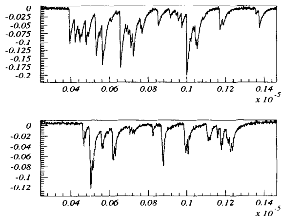
Fig. 2. A simulated signal (top) and a signal acquired in experimental condition very close to the simulated ones (bottom). The horizontal scale is in seconds, the vertical scale is pulse height in arbitrary units.
