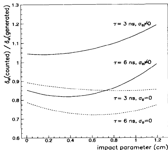
Fig. 3. Counting efficiency, for a cluster density of N_{cl} = 12 clusters/cm, as a function of the distance of closest approach of the track to the sense wire (impact parameter) for different values of \tau and \sigma_D .
