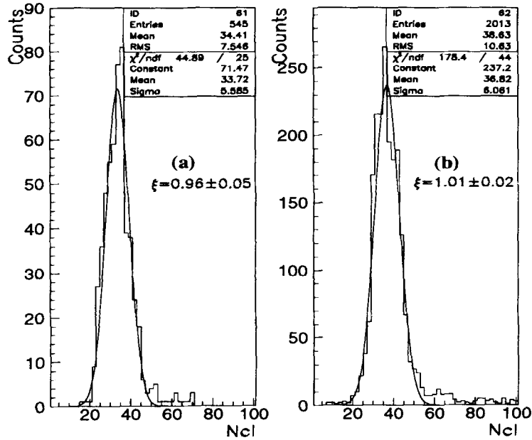
Fig. 12. Distribution of the number of clusters after an iterative application of the correction factor. The pion beam has a momentum of 280 MeV/c. Two different mixtures are shown: (a) 80%He 20% CH 4 and (b) 95%He 5% iC 4 H 10 .
