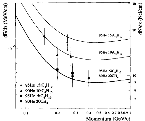
Fig. 17. Bethe-Bloch parameterization of dE/dx for pions, superimposed to the experimental data.
