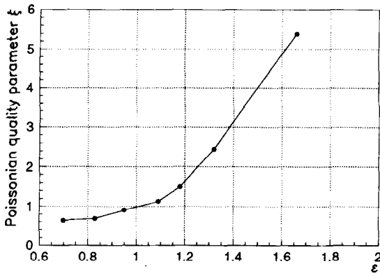
Fig. 5. For a simulated cluster density of 12/cm the quality parameter \xi , defined in the text, is plotted versus the ratio of counted over generated clusters, \epsilon . Each point corresponds to a different simulated dead time.
