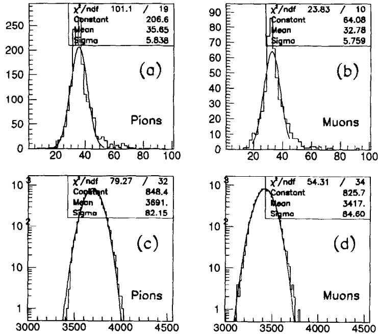
Fig. 13. Cluster distributions from single cell measurements ((a) pions, (b) muons) and for 100 cells sampling a track ((c) pions, (d) muons). Data refer to 200 MeV/c beam momentum and 95%He 5%iC 4 H 10 gas mixture.
