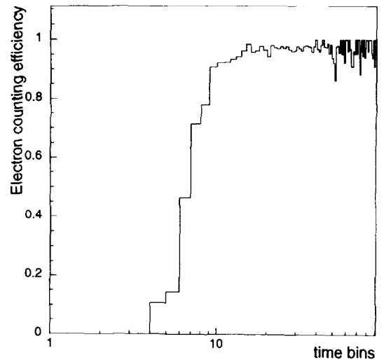
Fig. 10. The algorithm efficiency for resolving cluster pulses versus the distance (in bins) of each pulse from the previous one.
