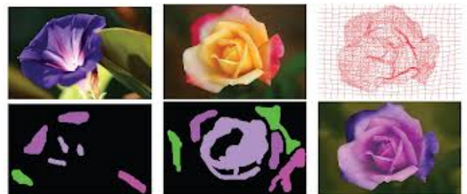
Figure 1 image features
