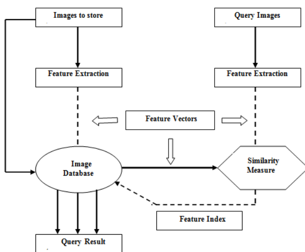
Figure 2 General Image Retrieval System
