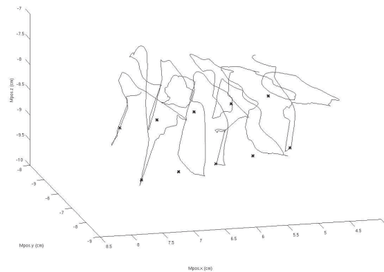
Fig. 11. Tool tip trajectory for Task 2 (touch each dot with left hand) while operating through UAV. The x's represent the location of each dot.
