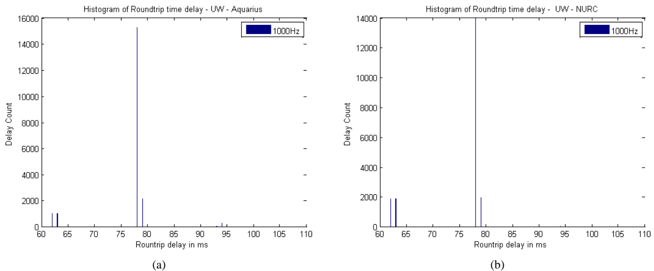
Fig. 16. Histogram of packets with respect to delay between (a) UW and Aquarius and (b) UW and NURC.
