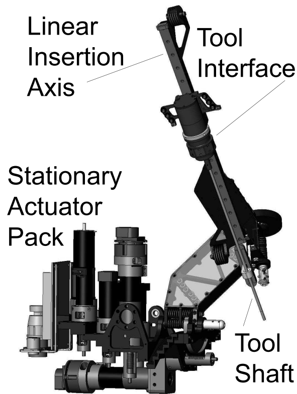
Fig. 5. CAD rendering of surgical manipulator shown with plastic covers removed. Mass: 12.3kg; folded dimensions 61cm x 53cm x 38cm; extended dimensions: 120cm x 30cm x 38cm.
