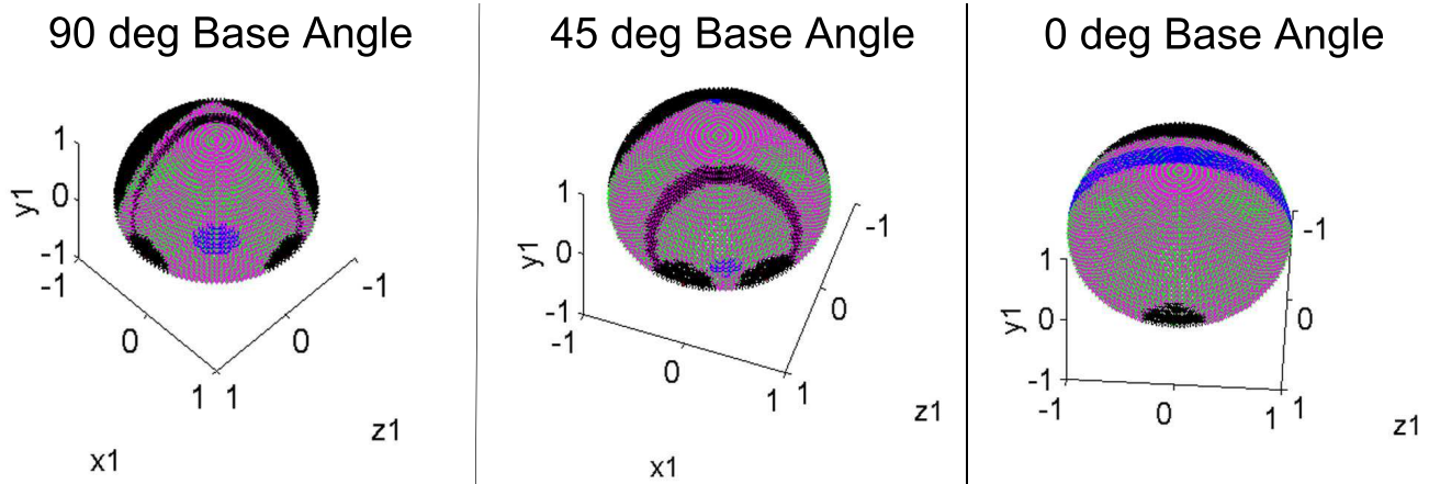
Fig. 4. The workspace is shown for the parallel mechanism with four equal link lengths of 60^\circ as a function of three different base angle \alpha_{12} = 90^\circ, 45^\circ, 0^\circ . Black represents areas outside the reachable workspace or areas near kinematic singularity. The circular area in the center of the workspace for the 90^\circ and 45^\circ bases and the stripe for the 0^\circ base represent an area of greatest isotropy. Notice that for the 90^\circ and 45^\circ bases and area of singularity cuts through the reachable workspace, a property that is highly undesirable.
