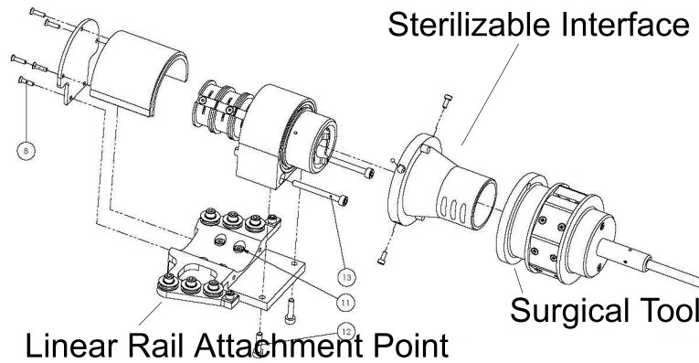
Fig. 6. Line drawing of tool interface, exploded view.
