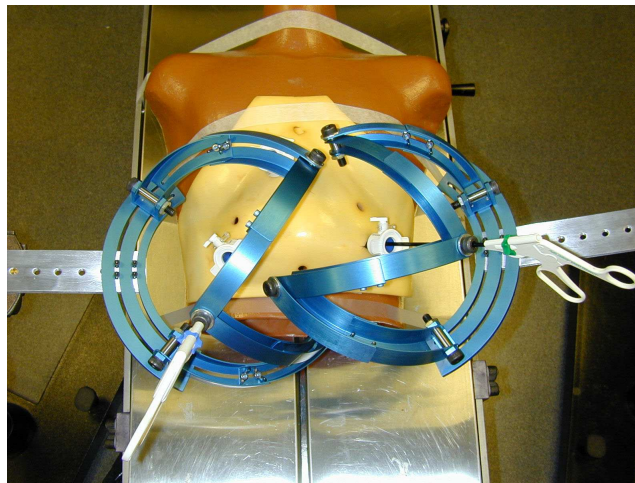
Fig. 2. Two parallel mechanism aluminum mock-ups. The parallel mechanism has four links and would have two actuated joints (the two base joints) if used for a surgical robot. It is clear from this picture that the parallel mechanism suffers from collision problems. The dry-lab experiments underscored the need for the most compact mechanism possible.
