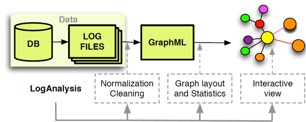
Fig. 1 Architecture of LogAnalysis .
